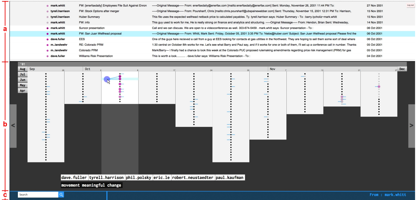
Figure 1: Overview of the mailVis interface showing (a) email display, (b) timeline visualization with 200 emails and (c) query field areas.
