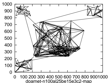
Figure 3.18: \alpha = 0.25, \beta = 0.15
