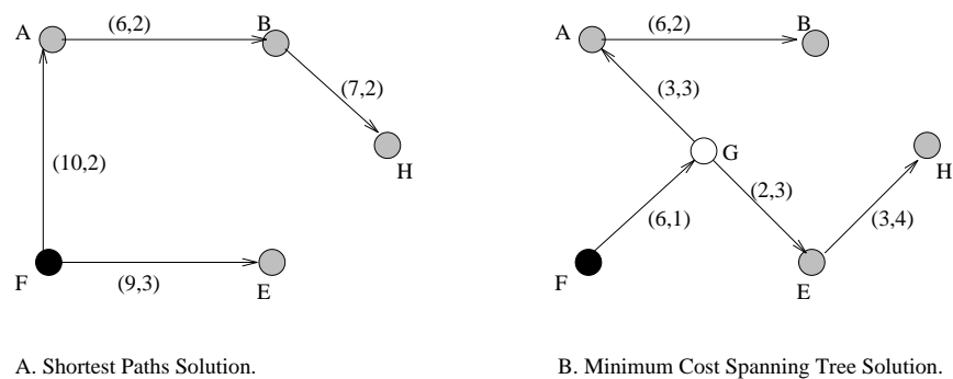
Figure 3.15: Benchmark solutions
