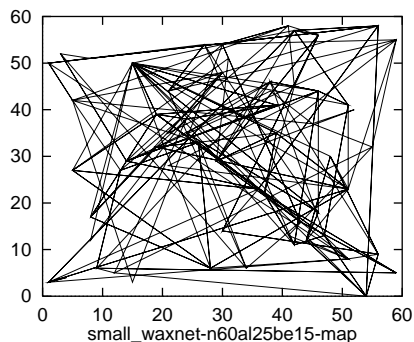
Figure 3.16: \alpha = 0.25, \beta = 0.15
