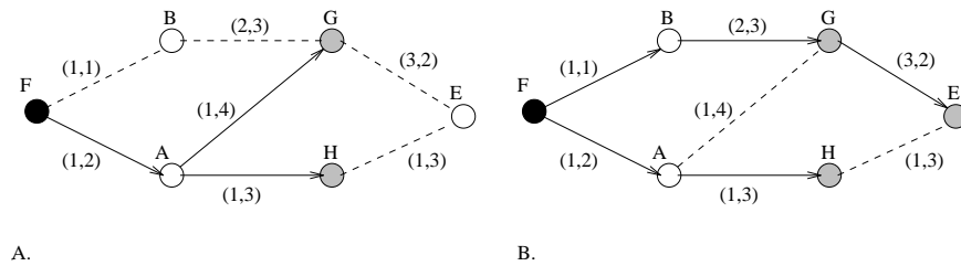
Figure 3.14: Changing topology of CSPT multicasts
