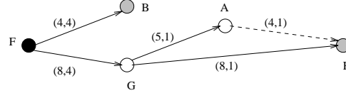
Figure 3.5: Costs increase as \Delta is relaxed. Figure 3.6: CCET more expensive than SPT.
