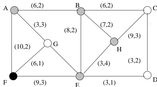
Figure 3.1: The example network
