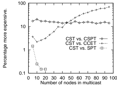
Figure 3.28: Effect of different delay bounds on CCET
