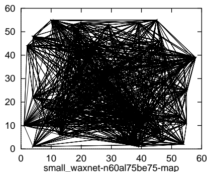
Figure 3.17: \alpha = 0.75, \beta = 0.75
