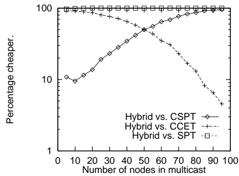
Figure 4.8: Hybrid cost saving
