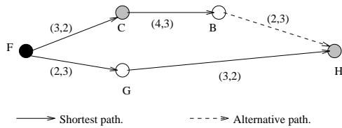
Figure 3.5: Costs increase as \Delta is relaxed. Figure 3.6: CCET more expensive than SPT.
