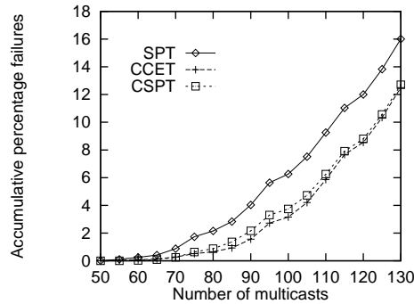
Figure 3.29: Network load and multicast failures
