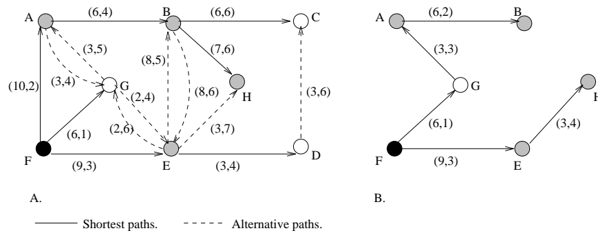
Figure 3.2: The CCET heuristic
