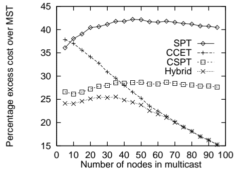
Figure 4.5: \Delta = multicast delay bound.
