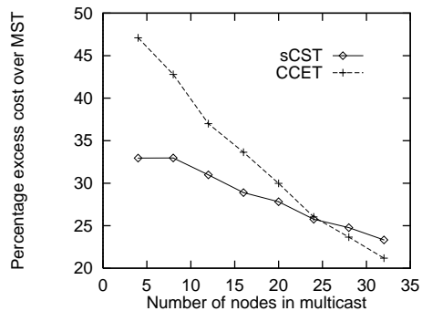
Figure 3.33: Cost performance of sCST c verses CCET
