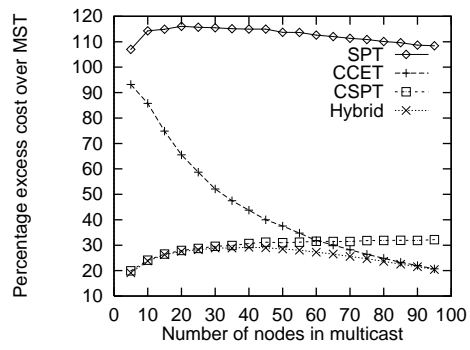
Figure 4.4: \Delta = MST delay bound
