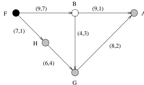
Figure 3.13: CSPT more expensive than SPT.
