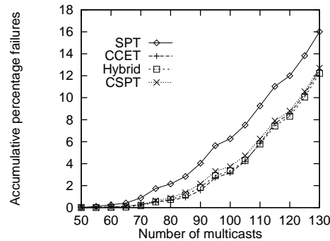
Figure 4.10: Network load and multicast failures
