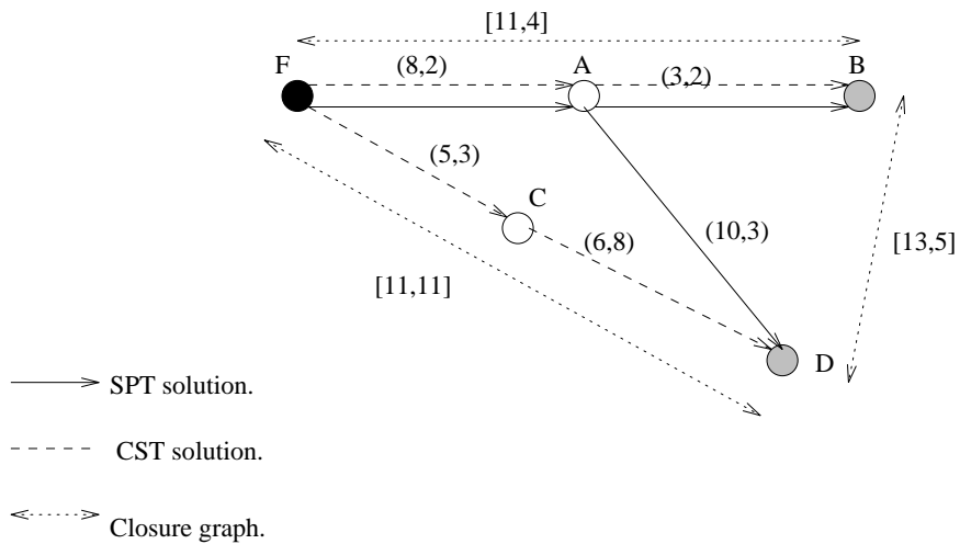
Figure 3.9: CST_c more expensive than SPT
