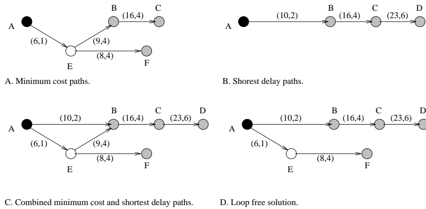
Figure 3.12: Loop removal in the CSPT heuristic
