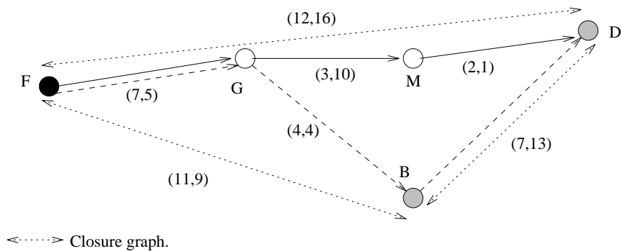
Figure 3.10: Changing topology of CST_c multicasts
