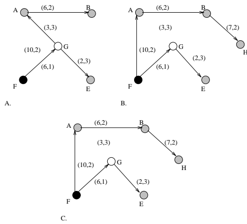
Figure 3.11: The CSPT heuristic
