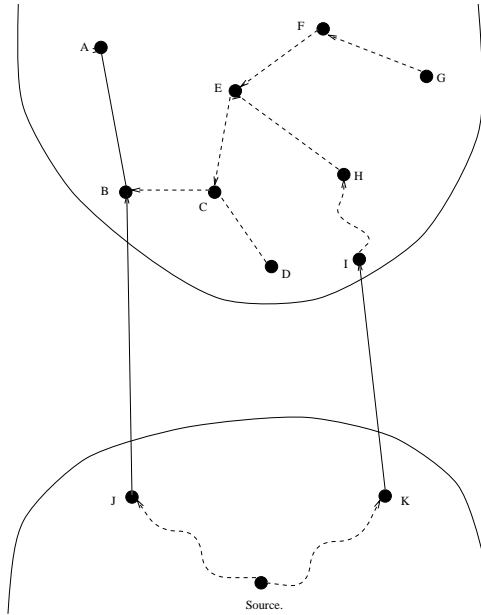
Figure 3.4: Rogue Paths and the Pathological Walkabout
