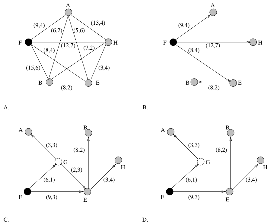
Figure 3.8: The CST_c heuristic
