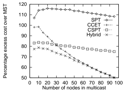
Figure 4.3: \Delta = multicast delay bound
