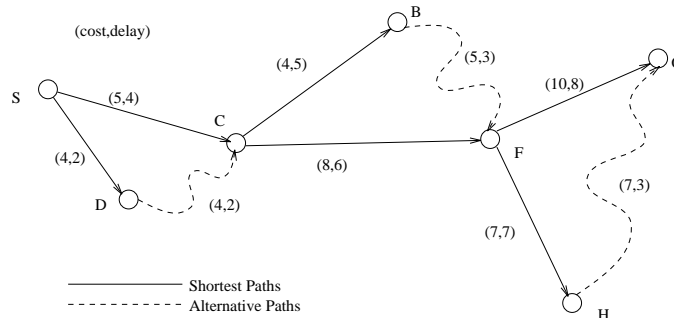
Figure 3.3: Example of a Rogue Path
