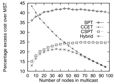
Figure 4.6: \Delta = network diameter
