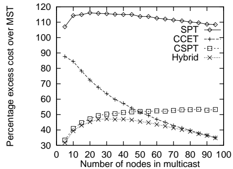
Figure 4.2: \Delta = network diameter.
