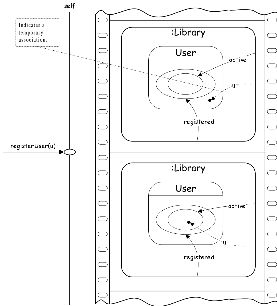
Figure 12: Generalised filmstrip for registerUser
