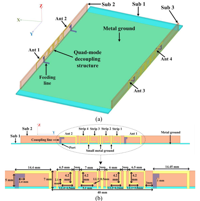
Fig. 9. Configuration of the 4-antenna array. (a) Overall view. (b) Detailed dimensions.
