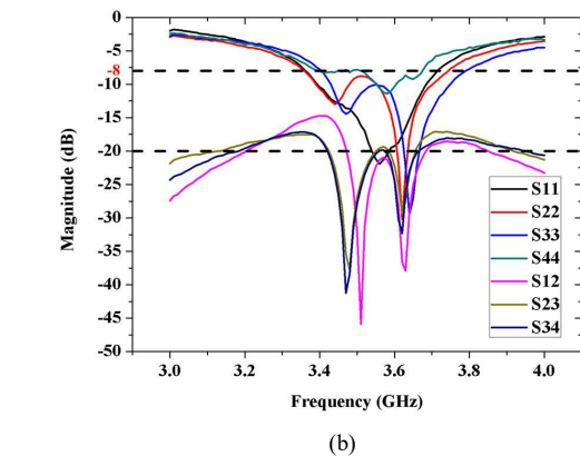
Fig. 8. (a) Fabricated prototype. (b) Measured S-parameter.
