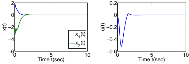
Fig. 6. Time responses of the system (2) under the Non-PDC integral sliding mode controller (55)
