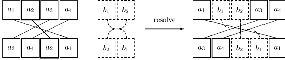
Figure 2. The derived permutation \varrho for the resolvent
