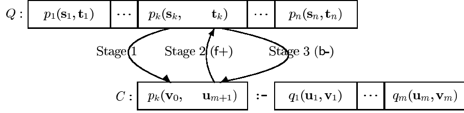
Figure A1. Data flow in the unification
