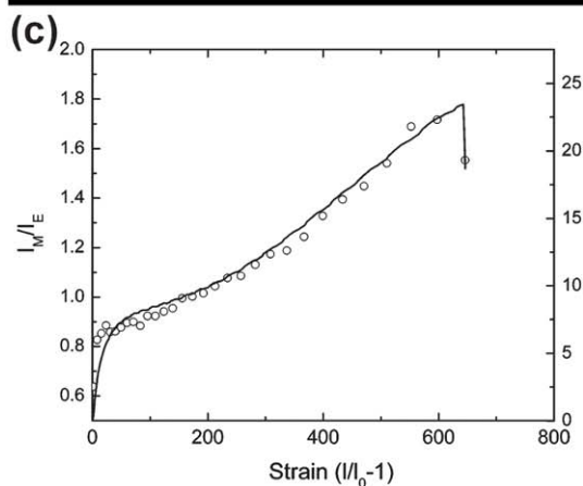
Fig. 18 (a) Synthesis of fluorescently labelled thermoplastic urethanes (TPUs MP1–MP7 and SP1–SP5 ). (b) Pictures (taken under excitation with UV light of a wavelength of 365 nm) of a film of MP6 in top, unstretched and bottom stretched state. (c) Ratio of monomer to excimer emission, I_M/I_E (circles, measured at 540 and 650 nm), and tensile stress (solid line) as a function of strain for films of SP4 . Reproduced with permission from ref. 42. © 2006 American Chemical Society.
