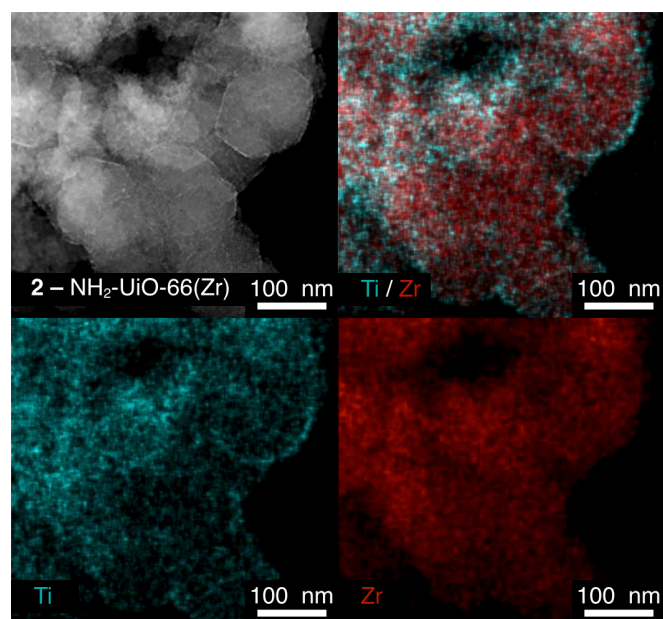
Figure 4. Transmission electron microscopy / energy dispersive X-ray spectroscopy images of \text{NH}_2\text{-UiO-66(Zr)} ( 2 ). Ti(IV) is present throughout the crystal, with highest concentrations found on the crystal edges.
