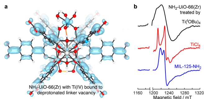
Figure 5. (a) The spin density of the pseudoexcited state of 16%- \text{NH}_2\text{-UiO-66(Zr)-Ti(OH)}_2(\text{H}_2\text{O}) , 2 shows a majority of spin contribution on the organic linker but, importantly a minor contribution from a Ti(III) d -orbital. The Ti(III) density should increase proportionally with loading on the framework. (b) Q-band continuous wave EPR spectra ( \approx 33.5 \text{ GHz} ) of photoexcited MIL-125- \text{NH}_2 , 1' and 2 in the reaction mixture of \text{CH}_3\text{CN}/\text{Et}_3\text{N}/\text{H}_2\text{O} .
