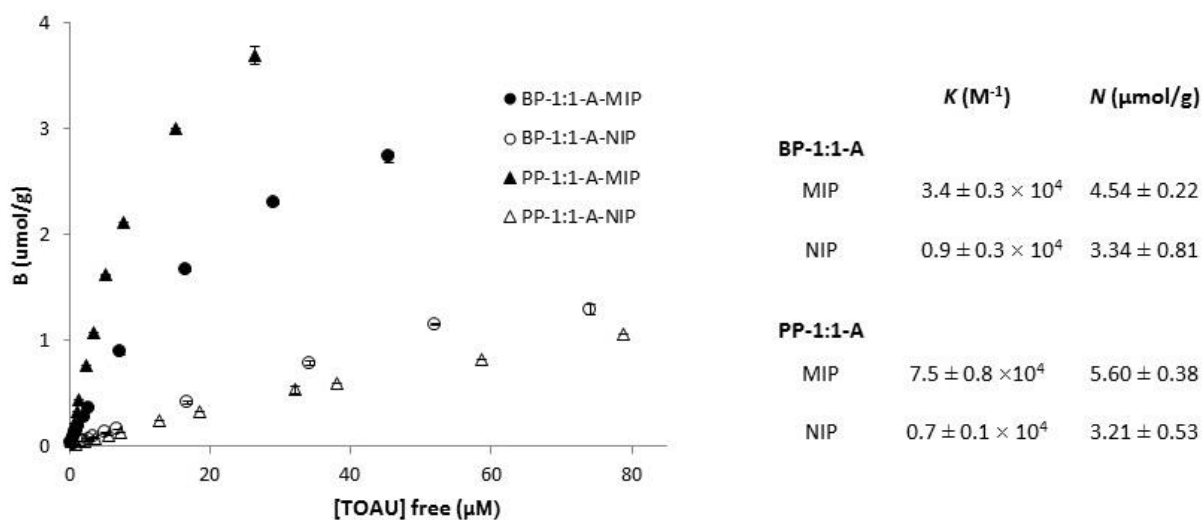
Figure 7. Binding isotherms of BP-1:1-A and PP-1:1-A polymers. Isotherms obtained using 10 mg polymer incubated for 1 hr in 0.500 mL of 1 to 100 \mu M TAU solution. Free TAU was measured by in-situ quantitative ^1 H NMR spectroscopy. Binding affinity constants ( K ) and number of binding sites were estimated from Prism GraphPad using the one-site hyperbola model. Errors are at 95% confidence level.
