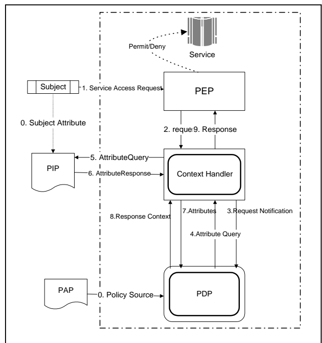
Figure 2 XACML Access Control Model
