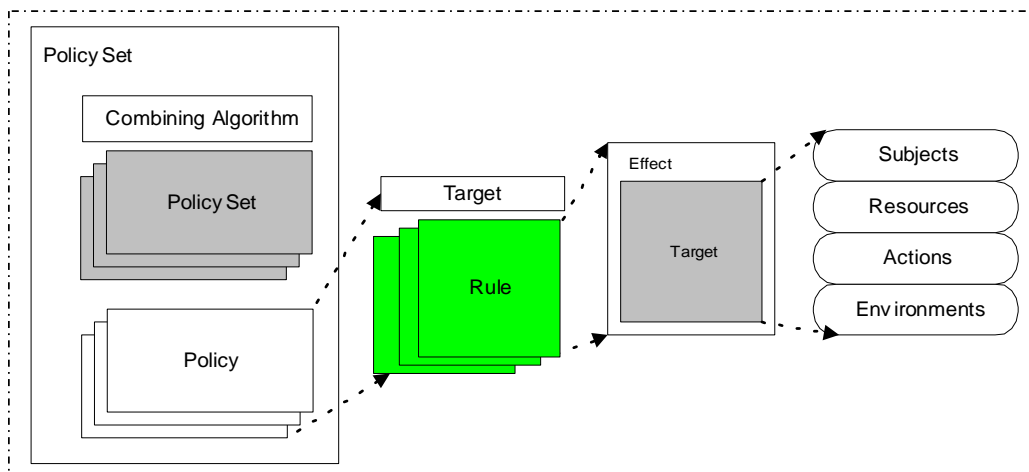
Figure 3 XACML Policy Language Structure
