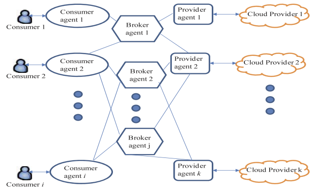
Fig. 5. An agent-based testbed for simulating cloud commerce.
