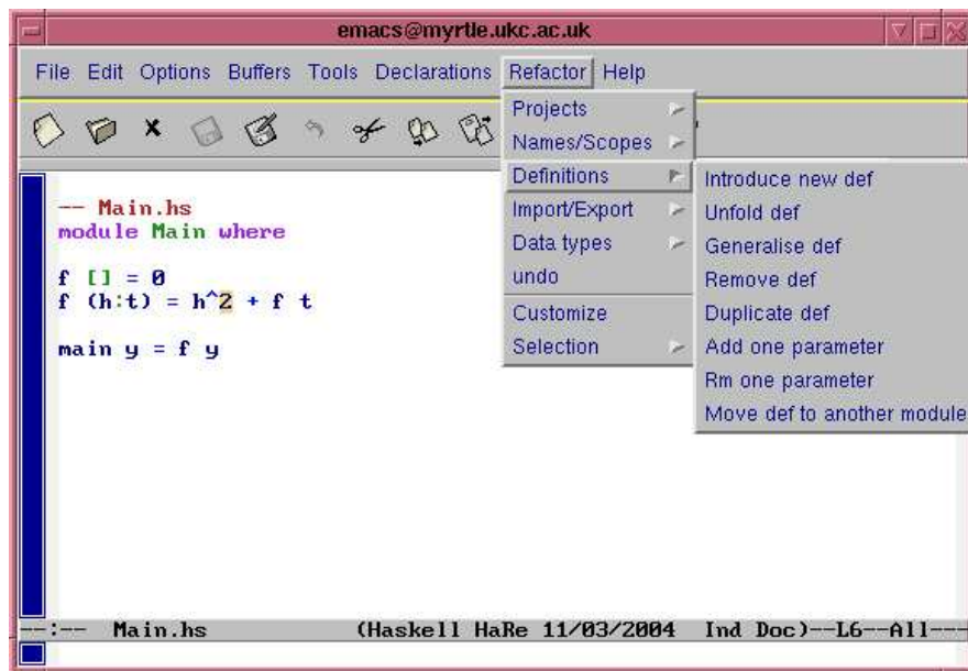
Figure 11: A snapshot showing the application of generalising a definition
