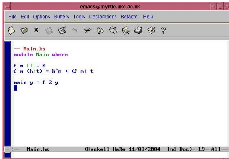
Figure 13: A snapshot showing the result of generalising a definition
