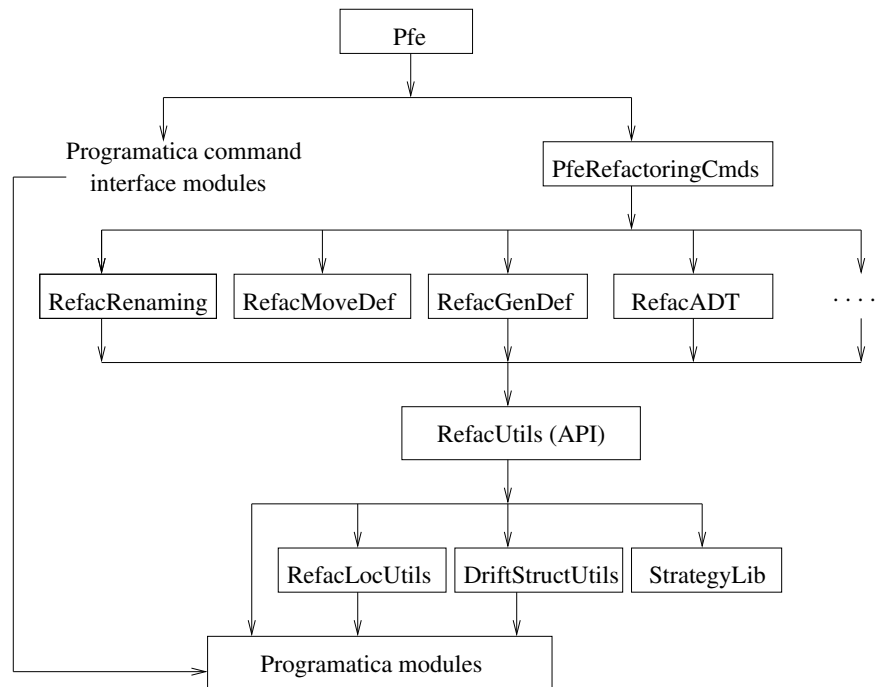
Figure 15: The module hierarchy of HaRe
