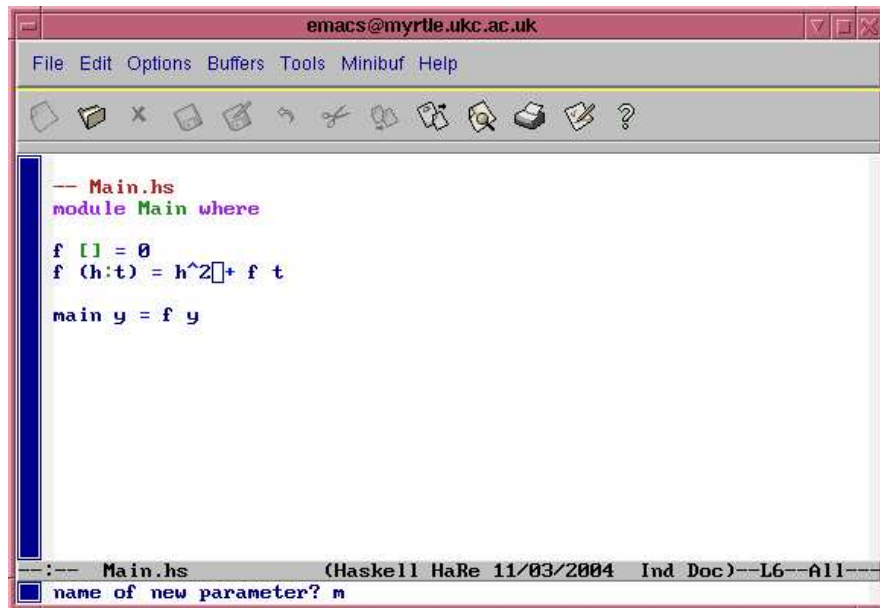
Figure 12: A snapshot asking for the parameter name during generalisation
