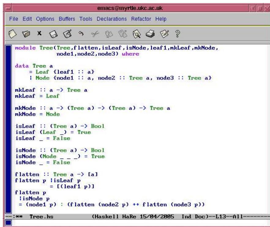
Figure 19: After applying from concrete to abstract data type to data type Tree
