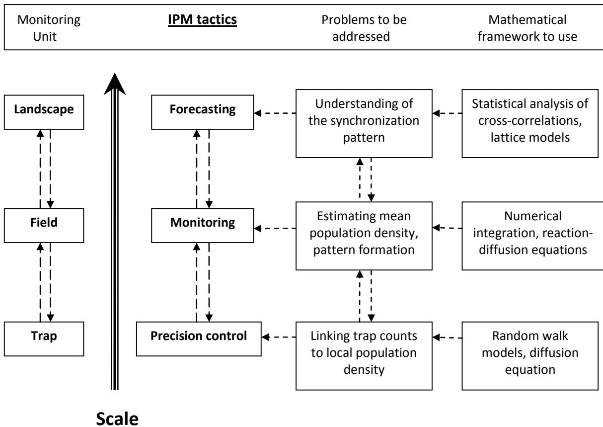
Figure 37: A sketch of the scale-specific goals of insect pest monitoring, corresponding theoretical frameworks and mathematical tools. The arrows indicate the information flow between different scales and approaches; see details in the text.
