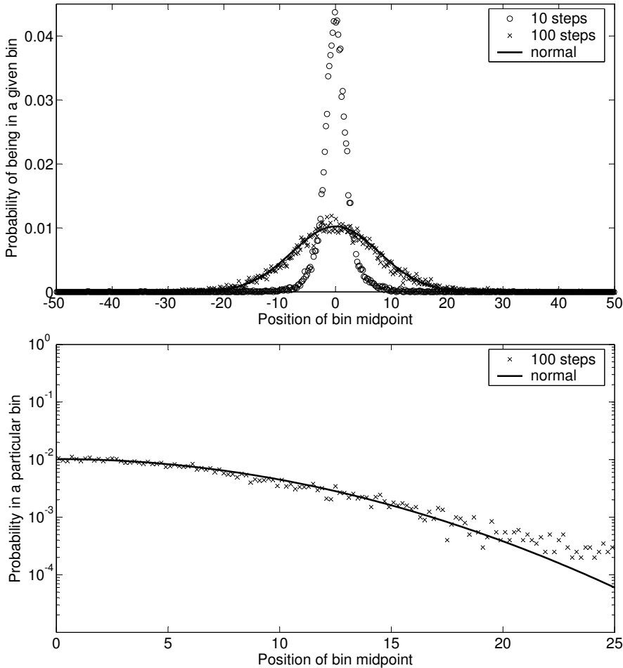
Figure 8: Probability density distribution for the position of a random walker obtained in individual-based simulations after 10^4 realizations. At t = 0 the walker is released at x = 0 . The symbols show the probability density given by the frequency per unit length in the interval or ‘bin’ centered at a given location x ; the bin width is \Delta x = 0.2 . The dispersal kernel used is \varrho = C(|\xi| + \gamma)^{-\alpha} where C = 0.5(\alpha - 1) , \alpha = 3.5 and \gamma = 1 . (top) The emerging spatial distribution after 10 steps (circles) and after 100 steps (crosses). The solid curve shows the normal distribution \mathcal{N}(0, 7.8) . (bottom) A fragment of the total domain showing the tail of the distribution emerging after 100 steps (in semi-logarithmic coordinates). Clearly there is a considerable deviation between the normal distribution and the actual population distribution at large x .
