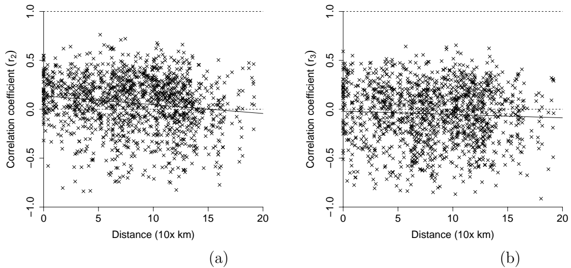
Figure 34: Plots of correlation coefficients for pairs of distinct fields against distance between those fields calculated using the time-lag of (a) 2 years, (b) 3 years. The solid lines indicate trends predicted by linear regression analysis.
