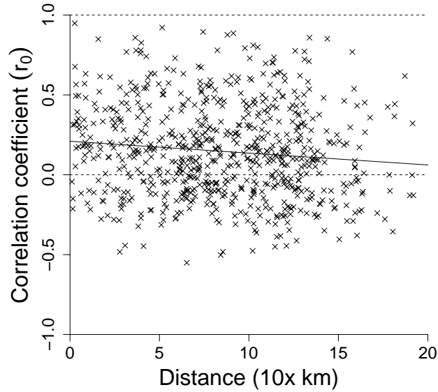
Figure 29: Plot of the correlation coefficients, see Eq. (91), for pairs of fields against distance between those fields. The solid line indicate the trend predicted by the linear regression analysis.
