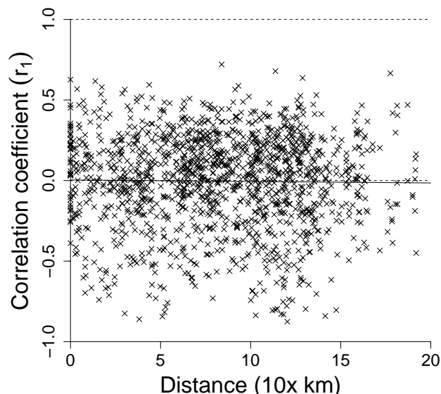
Figure 31: Plots of correlation coefficients r_1 for pairs of distinct fields against distance between those fields calculated using the time-lag of 1 year, cf. Eq. (93) with k = 1 . The solid line indicate the trend as predicted by linear regression analysis.
