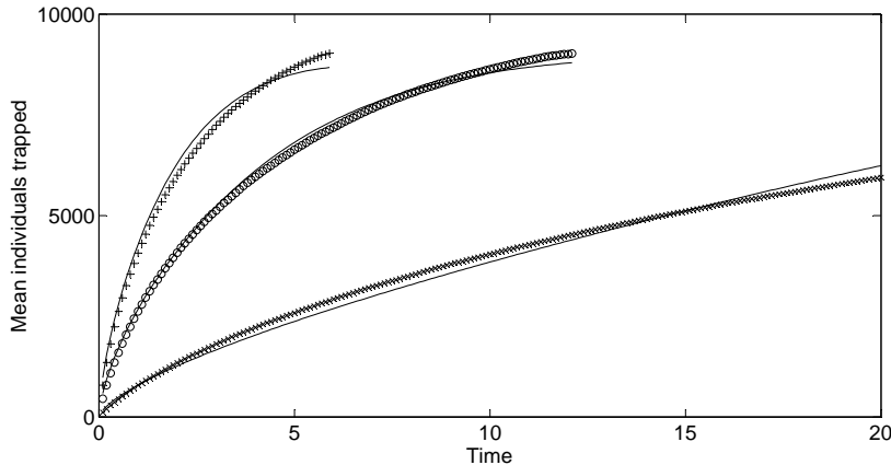
Figure 18: Time dependent diffusion curves fitted to Levy walk trap counts, where H = 1/3 , and b is determined from the first datapoint (at t = 0.1 ).
