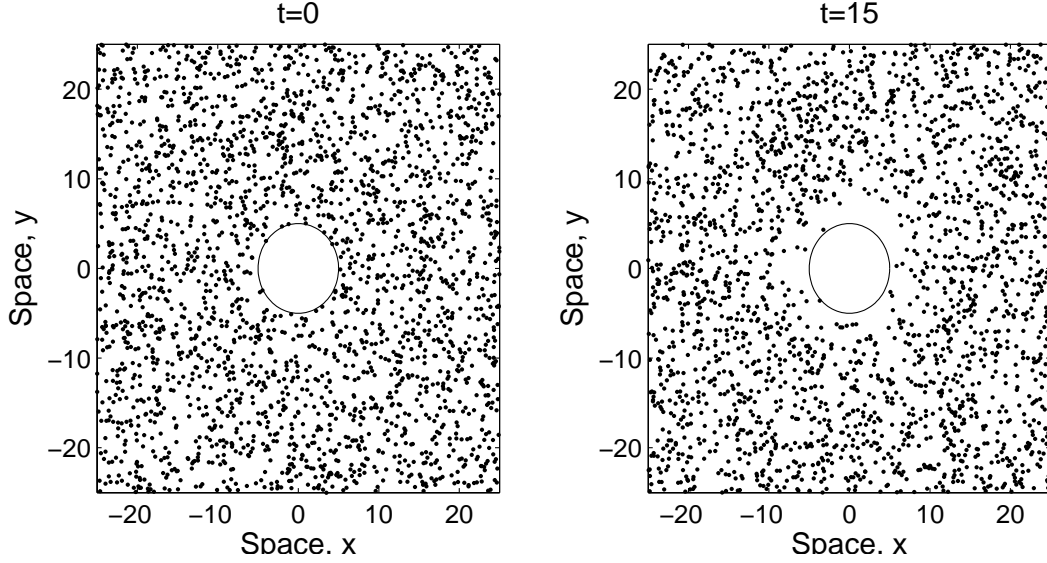
Figure 3: Population of insects performing the Brownian motion as defined by (1) with \delta^2 = 0.02 ; snapshots are shown at t = 0 (left) and t = 15 (right), i.e. after 1500 steps with a hypothetical value \Delta t = 0.01 . Only a part of the computational domain is shown, the total size is 100 \times 100 . The initial population density is U_0 = 1 which corresponds to the total initial population size of K = 10^4 .
