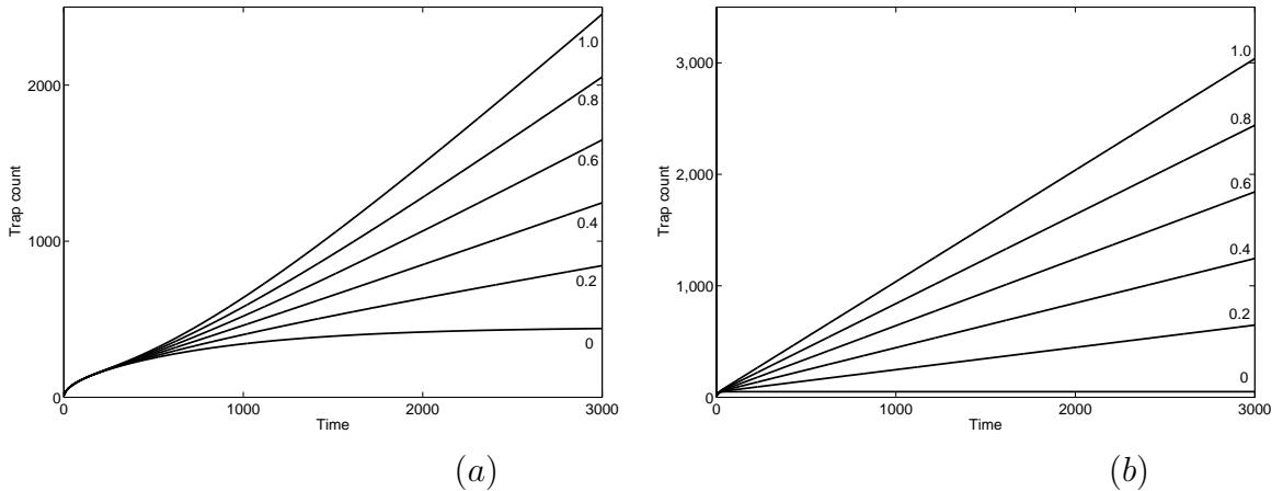
Figure 12: Trap count vs time in case of the Neumann-type boundary forcing, see Eq. (43), for the initial population density U_0 = 10 and for different size of the domain, (a) for L = 45 , (b) for L = 5 . Different curves correspond to different values of the gradient G as it varies between 0 and 1 (bottom to top, respectively).
