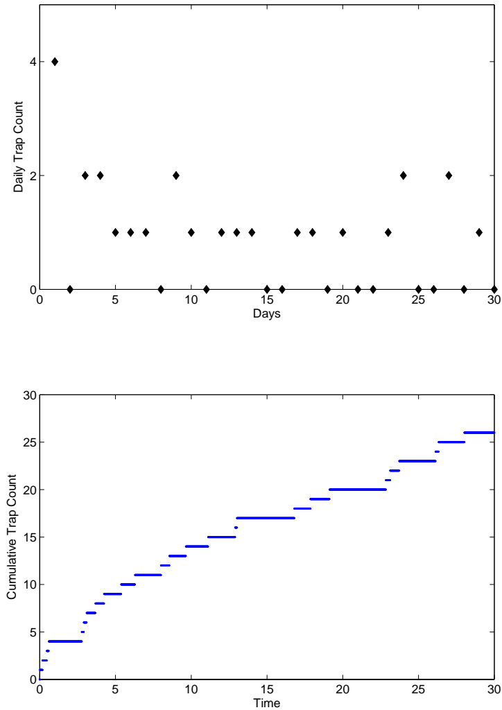
Figure 5: Trap counts vs time (in days) obtained for U_0 = 0.1 (which corresponds to the total initial population size of K = 10^3 insects), other parameters as in Fig. 3. Top: daily trap count C ; bottom: the cumulative number J of the insects trapped, see Eq. (8).
