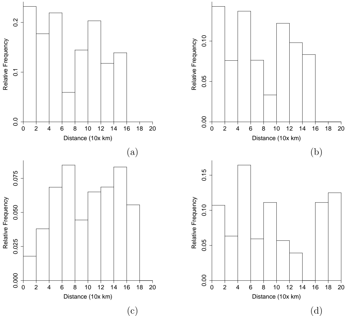
Figure 36: Distribution of distances between significantly correlated fields as obtained for (a) r_0 , (b) r_1 , (c) r_2 and (d) r_3 , i.e. for the time-delay of none, one, two and three years, respectively. The corresponding mean distance is 72.9, 74.9, 100.0 and 94.7 kms.
