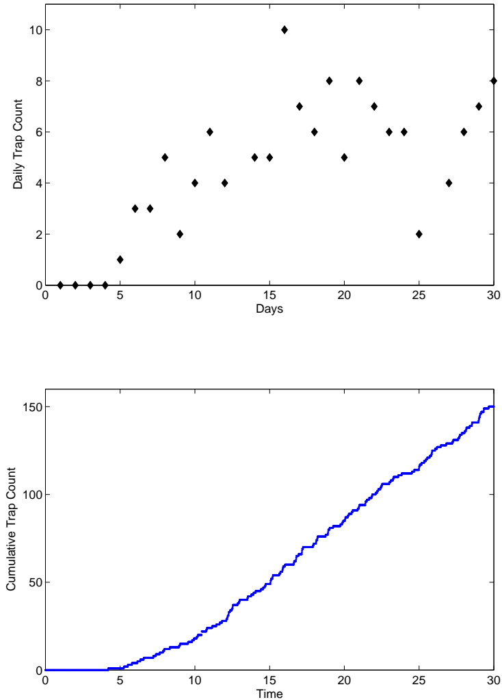
Figure 7: Trap counts vs time (in days) obtained for the point-source release with parameters as in Fig. 6. Top: daily trap count C ; bottom: the cumulative number J of the insects trapped, see Eq. (8).
