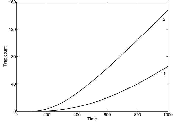
Figure 15: Trap counts obtained for parameters D = 1 , L = 45 , U_b = 10 , U_0 = 0 . Curve 2 for the Dirichlet-type boundary forcing, curve 1 curve for the Neumann-type boundary forcing with G = U_b/L = 0.45 .
