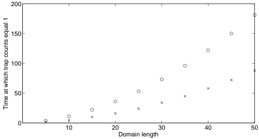
Figure 16: Plot of time t_1 (y-axis) at which trap counts J(t_0) = 1 against length of domain (x-axis). Crosses for the Dirichlet-type forcing, circles for the Neumann-type forcing. Parameters are: D = 1 , U_0 = 0 , U_b = 10 and G = U_b/L .
