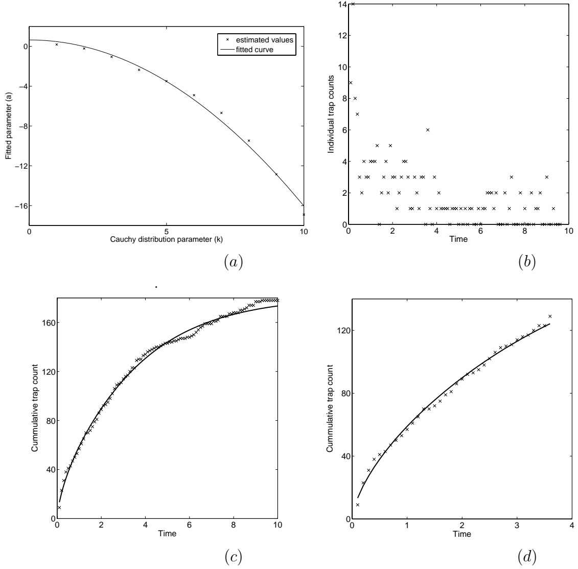
Figure 19: (a) Variation of parameter a with k . The solid curve is the best-fitting quadratic polynomial. (b) the daily trap counts obtained for the Levy-walking population (60–61) that at t = 0 is distributed uniformly (in the statistical sense) over the domain 0 < x < 20 with the mean density U_0 = 10 ; (c) the corresponding cumulative trap counts (shown by crosses) and their best-fit (shown by the solid curve) by the mean-field model with time-dependent diffusion, the best fit is obtained for U_0 = 9.7 ; (d) the results of data fitting in case of a smaller dataset, the best fit is obtained for U_0 = 9.3 .
