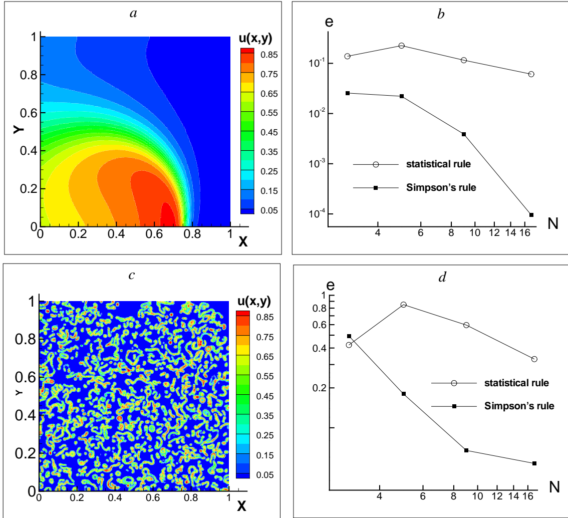
Figure 23: The coarse grid problem in the 2D case. (a,c) Population density u(x, y) obtained from a mathematical model of population dynamics (see details in the text), (b,d) the corresponding integration error (76) shown on the logarithmic scale, N is the number of nodes in each direction x and y of a regular Cartesian grid. (a) A single peak population distribution typical for the values of the diffusion coefficient D \sim 1 or larger. (b) The integration error for the statistical rule (solid line, open circle) and the Simpson rule (solid line, closed square) corresponding to (a). (c) A snapshot of the patchy population density distribution typical for D \ll 1 . (d) The integration error corresponding to (c), the legend as the same as in Fig. 23b.
