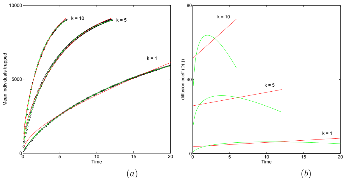
Figure 17: (a) Trap counts simulated for Levy walks as given by (60–61) (different symbols correspond to different values of k ) and their approximation with time-dependent diffusion for linear D(t) (red curves) and nonlinear D(t) (green curves). Simulations were stopped when the number of trapped insects reached 90% of the total population. (b) The diffusion coefficient D as a function of time for the simulations shown in (a). At t = 0 the population of K = 10^4 insects is distributed uniformly over the domain of size L = 20 .
