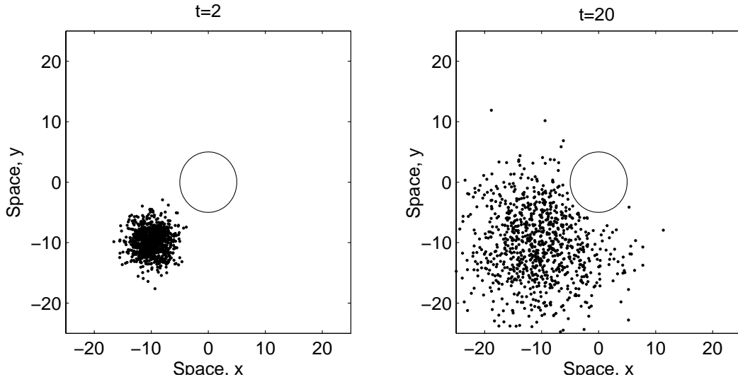
Figure 6: Population of insects performing the Brownian motion (Eqs. (1) with \delta^2 = 0.01 ); snapshots are shown at t = 2 (left) and t = 20 (right), i.e. after 200 and 2000 steps, correspondingly. Only a part of the computational domain is shown. The initial population consists of K = 10^3 insects and is released at the point (x, y) = (-10, -10) .
