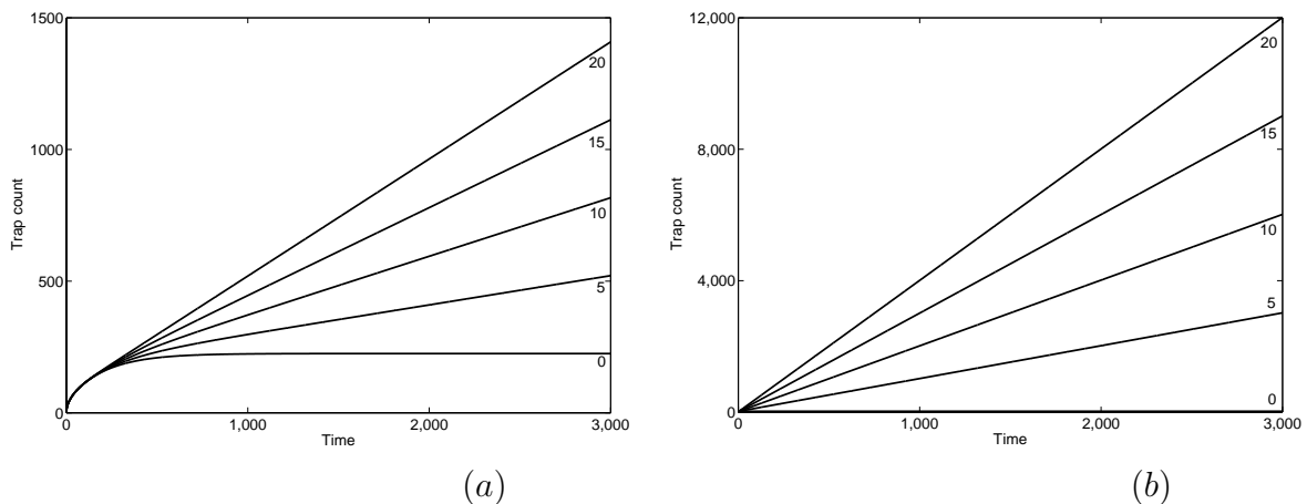
Figure 13: Trap count vs time in case of the Dirichlet-type boundary forcing, see Eq. (46), for the initial population density U_0 = 10 and for different size of the domain, (a) for L = 45 , (b) for L = 5 . Different curves correspond to different values of U_b as it varies from 0 to 20 (bottom to top, respectively).
