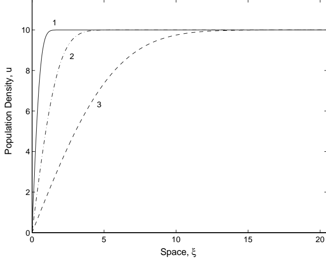
Figure 9: Population density vs space as given by the solution (33) of the diffusion equation (24) at t = 0.1 (solid curve 1), t = 1 (dashed-and-dotted curve 2) and t = 10 (dashed curve 3) for parameters D = 1 and U_0 = 10 . The diffusion equation is solved numerically in the domain 0 < x < L with L = 30 with the boundary conditions u(0, t) = 0 and \partial u(L, t)/\partial x = 0 .
