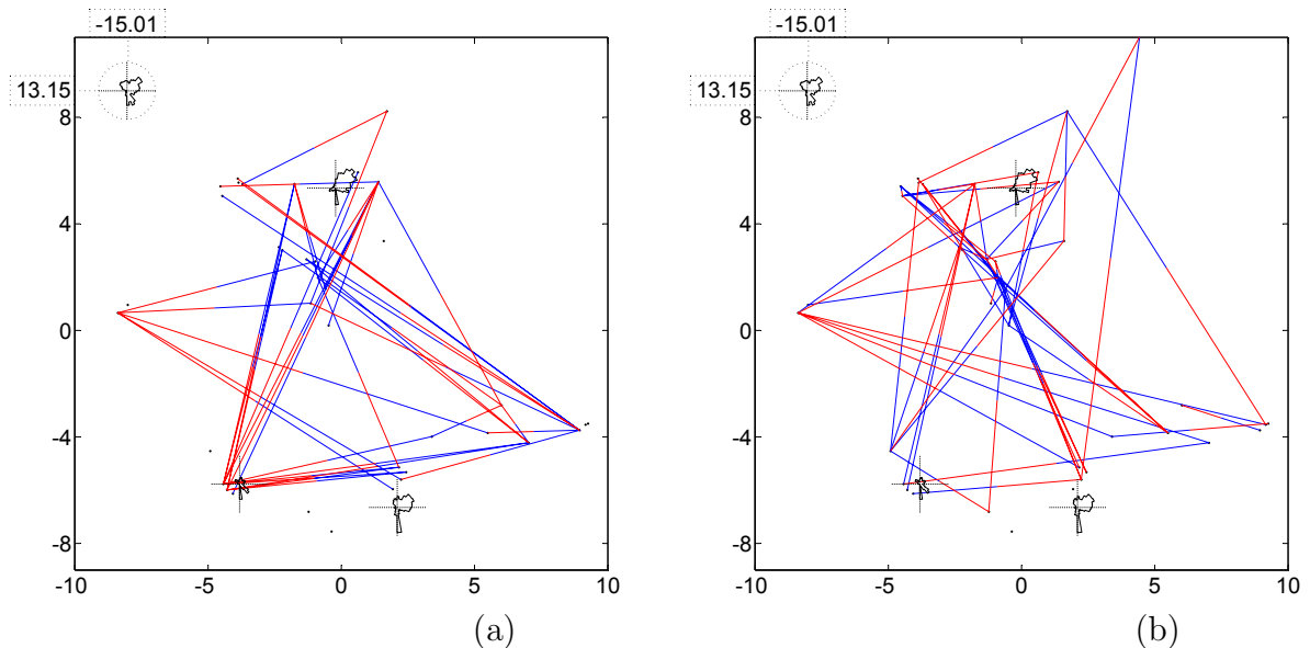
Figure 35: Network of significant inter-field correlations calculated using the time-lag of (a) 2 years, (b) 3 years. The red section of each line emanates from the influencing field, the blue section terminates at the influenced field.
