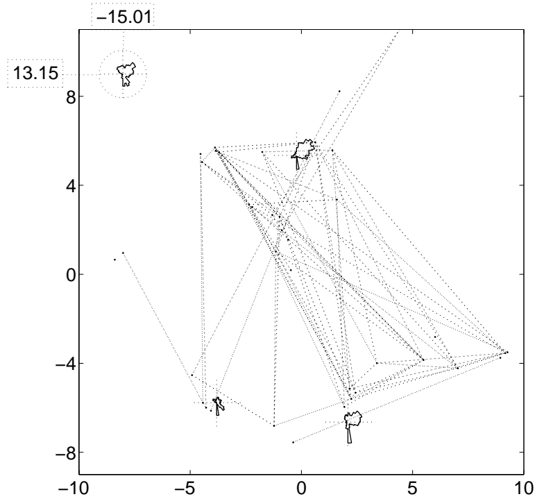
Figure 30: Network of inter-field correlations. The dotted lines connect fields with significantly correlated populations. Further details are given in the text. Scales indicate relative position in tens of kilometers. The inset (top-left corner) shows a weather station that is situated outside of the domain.
