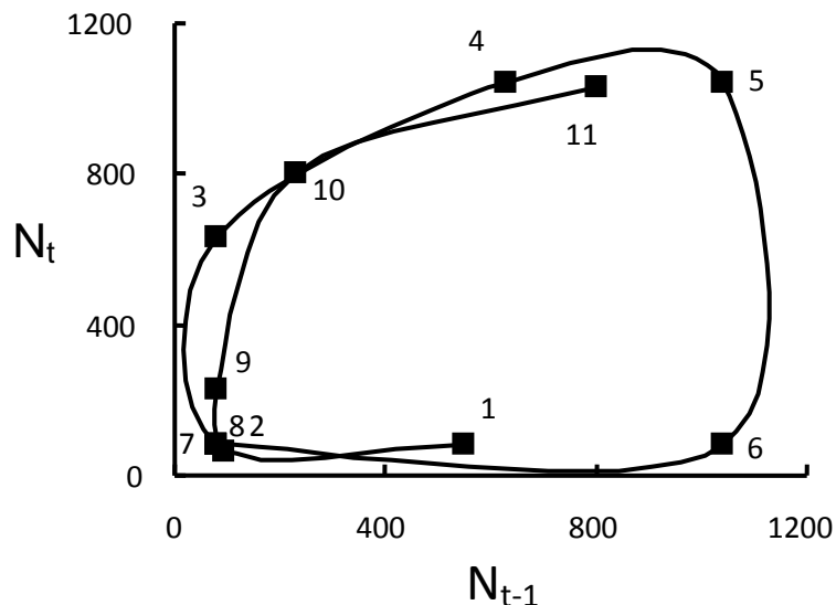
Figure 33: Phase trajectory of annual leatherjacket population ( \times 10^3 ) changes in south-west England. Each point is a plot of the population in the current year ( N_t ) against the population in the previous year ( N_{t-1} ). The line connects points in chronological order with points numbered sequentially. Data from Fig. 3 in [90].
