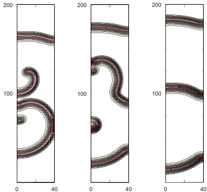
Figure 39: The population density of prey in a predator-prey system shown for three equidistant moments. As the time increases (from left to right), the irregular 2D pattern converges to an effectively 1D system of plane waves. From [98], with permissions.
