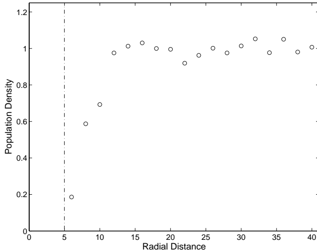
Figure 4: Insect density as a function of the radial distance from the center of the trap corresponding to the snapshot shown in Fig. 3, right. The vertical line shows the position of the trap boundary.
