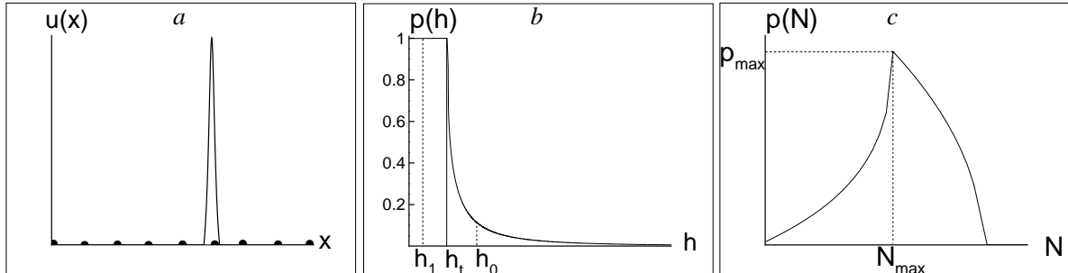
Figure 25: (a) An example of a 1D highly aggregated distribution of the population density u(x) (high density patch, peak function), black dots show the position of the grid nodes. (b) The probability of obtaining an accurate estimate of the pest population size in the case that traps are installed at nodes of a regular grid. (c) The probability of obtaining an accurate estimate of the pest population size using the integration rule (72-73) on a random grid of traps under the constraint that only a single trap falls into the high density patch.
