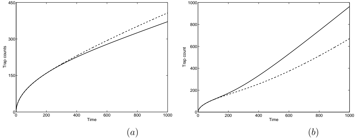
Figure 14: Trap counts obtained from for (a) U_b = 10 , and (b) U_b = 50 . Other parameters are D = 1 , L = 45 , U_0 = 10 and G = U_b/L . Dashed curve for the Neumann forcing, solid curve for the Dirichlet forcing, Eqs. (44) and (47) respectively.
