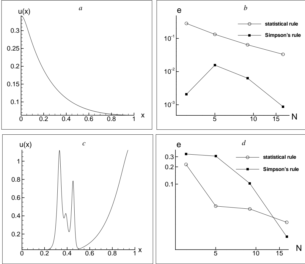
Figure 22: The coarse grid problem. (a) A monotone spatial distribution of the pest population density u(x) obtained for the diffusion coefficient D = 10^{-4} . Other parameters along with the initial and boundary conditions used to generate one-dimensional density distributions are discussed in [115]. (b) The integration error (76) arising from numerical integration of the distribution Fig. 22a using the statistical rule (72-73) (solid line, open circle) and the Simpson's rule (80) (solid line, closed square). The error is shown on the logarithmic scale. (c) A 'multi-peak' density distribution obtained for the diffusion coefficient D = 10^{-5} . (d) The integration error (76) corresponding to Fig. 22c, the legend as the same as in Fig. 22b.
