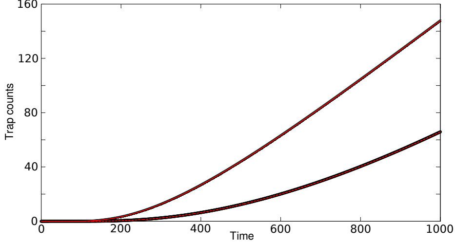
Figure 5: Trap counts vs time as given by the series (16) (upper curve) and (17) (lower curve), i.e. for diffusive and advective forcing respectively, and as obtained from numerical solutions of the corresponding systems. Parameters are: D = 1 , L = 45 , U_0 = 0 , U_b = 10 and G = U_b/L . Red curves correspond to the analytical solutions (truncated at 100 terms), black symbols correspond to numerical solutions. Note the excellent agreement between the analytical and numerical results.
