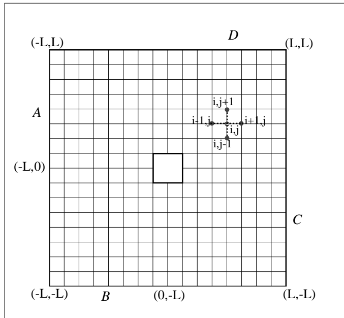
Figure 9: A computational grid in the domain \Omega_s . The trap is placed at the origin (0, 0) . The discretization of the equation (41) at the grid node n_{ij} requires the values of the function u(x, y, t) at the nodes n_{ij} , n_{i-1j} , n_{i+1j} , n_{ij-1} and n_{ij+1} . Letters A, B, C and D denote the domain edges where different boundary conditions can be used; see section 6.
