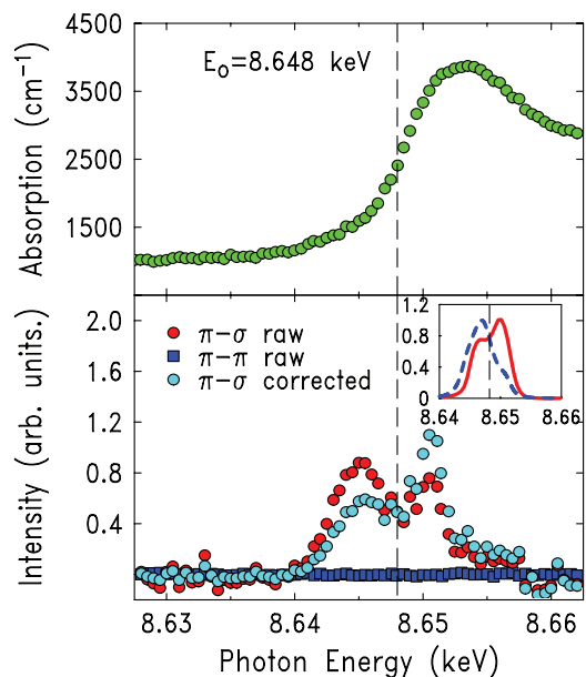
FIG. 2. (Color online) Tm absorption measured through a 5- \mu\text{m} -thick foil and rescaled to tabulated values (upper panel). The inflection point is labeled as E_0 . In the lower panel, we show the raw data for the (006- \tau ) magnetic reflection for both \pi \rightarrow \sigma and \pi \rightarrow \pi channels as well as the \pi \rightarrow \sigma absorption-corrected data. The inset of the lower panel shows the results of the relativistic DFT (red, solid) and also the simple model results that do not include the energy dependence of the matrix elements (blue, dashed).
