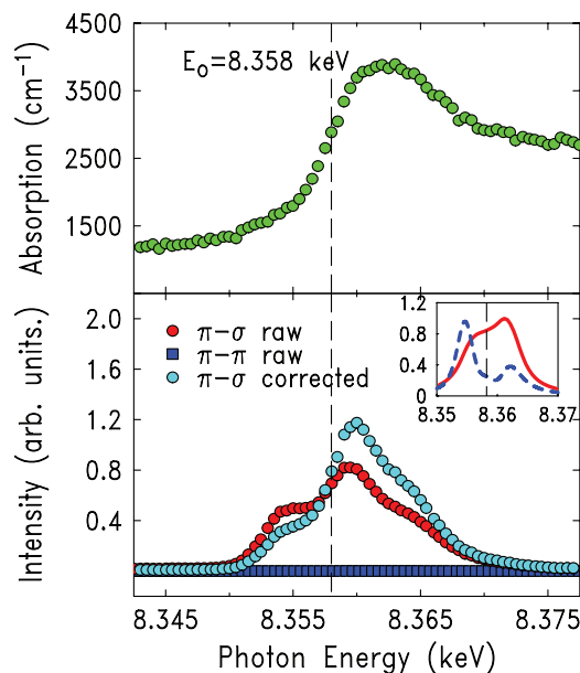
FIG. 1. (Color online) Er absorption measured through a 5- \mu\text{m} -thick foil and rescaled to tabulated values (upper panel). The inflection point is labeled as E_0 . In the lower panel, we show the raw data for the (006- \tau ) magnetic reflection for both \pi \rightarrow \sigma and \pi \rightarrow \pi channels as well as the \pi \rightarrow \sigma absorption-corrected data. The inset of the lower panel shows the relativistic DFT results (red, solid) and also the simple model results that do not include the energy dependence of the matrix elements (blue, dashed).
