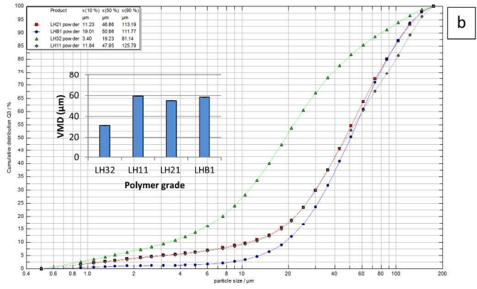
Hausner ratio and Carr's index of the LH32, LH21, LH11 and LHB1 polymers (a) and laser diffraction particle size analysis using (b).
