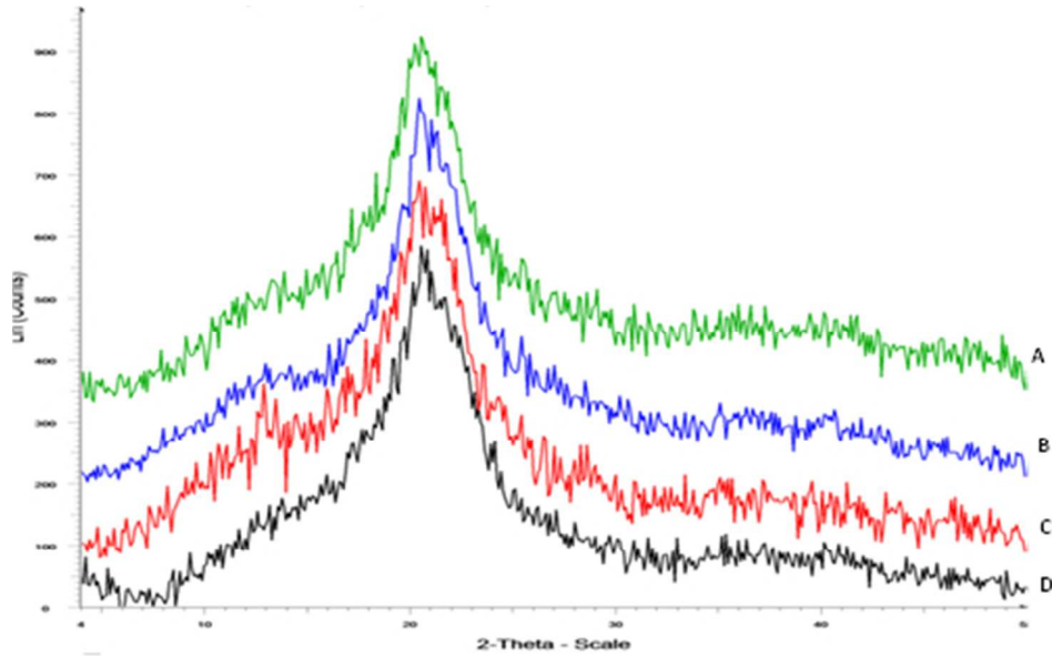
XRD diffraction pattern for LHB1 (A), LH32 (B), LH21 (C), LH11(D)
