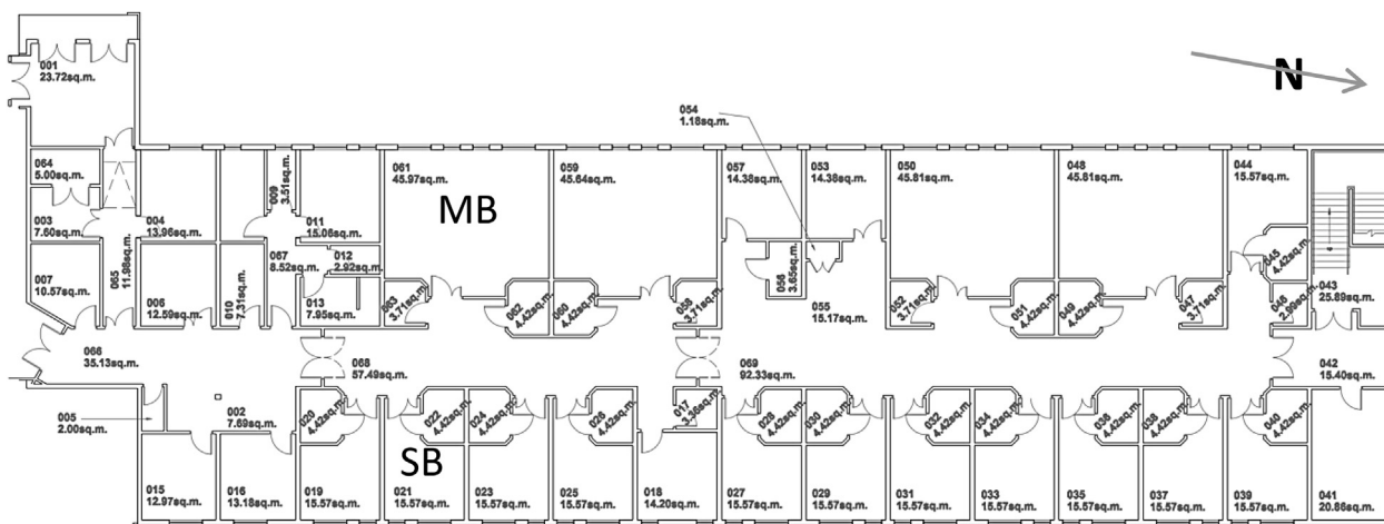
Fig. 3. Floor plan of the modular building. Single-bed (SB) rooms are along the east side and multi-bed (MB) rooms along the west side.
