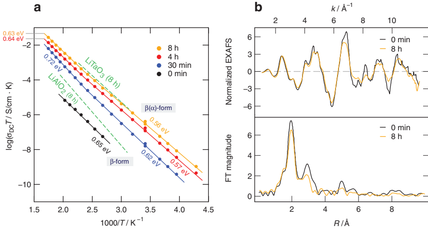
Fig. 21: (a) Arrhenius plot showing the temperature dependence of \sigma_{DC} T of micro- and nanocrystalline \beta - \text{Li}_2\text{TiO}_3 . Note that, according to X-ray diffraction, after 8 h of milling a mixture of amorphous \text{Li}_2\text{TiO}_3 , the \beta -form and the \alpha -modification has been formed. The dashed lines indicate conductivities of \text{LiTaO}_3 and \text{LiAlO}_2 each milled for 8 h, for comparison. (b) Normalized EXAFS data of the source material and the sample milled for 8 h in a planetary mill; (b) Fourier transforms (FT) of the k^3 weighted normalized EXAFS data shown at the top. The data were analyzed to yield details on the local structure, i.e. bond lengths, R , Debye–Waller factors, \sigma_{DW} . Figures taken from Refs. [27, 48].
