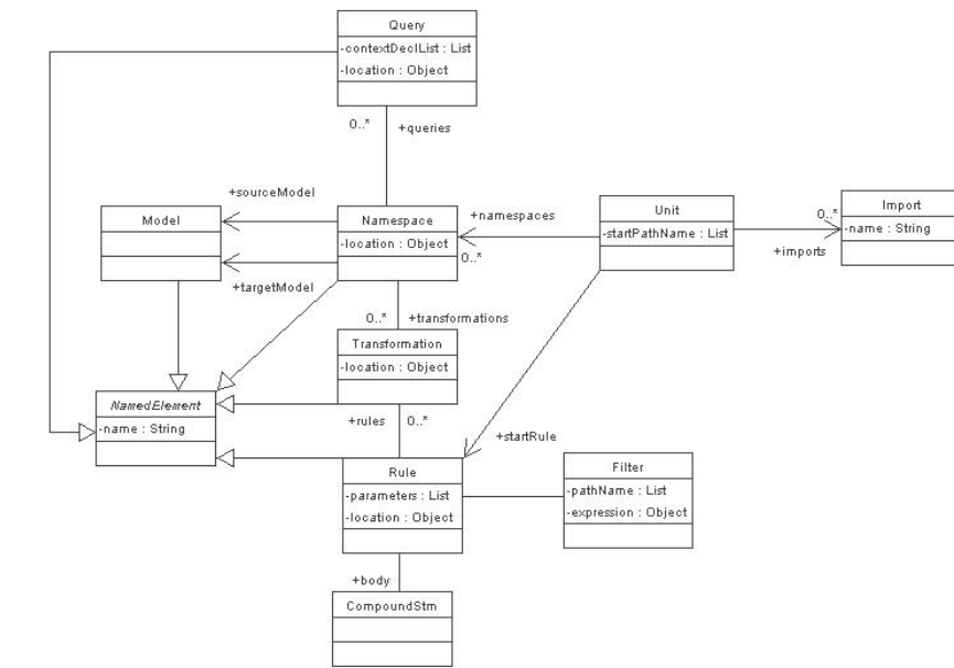
Figure 1 Abstract Syntax
