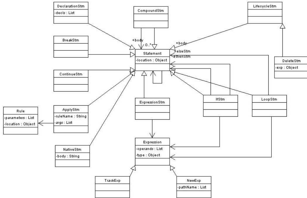
Figure 2 Statements
