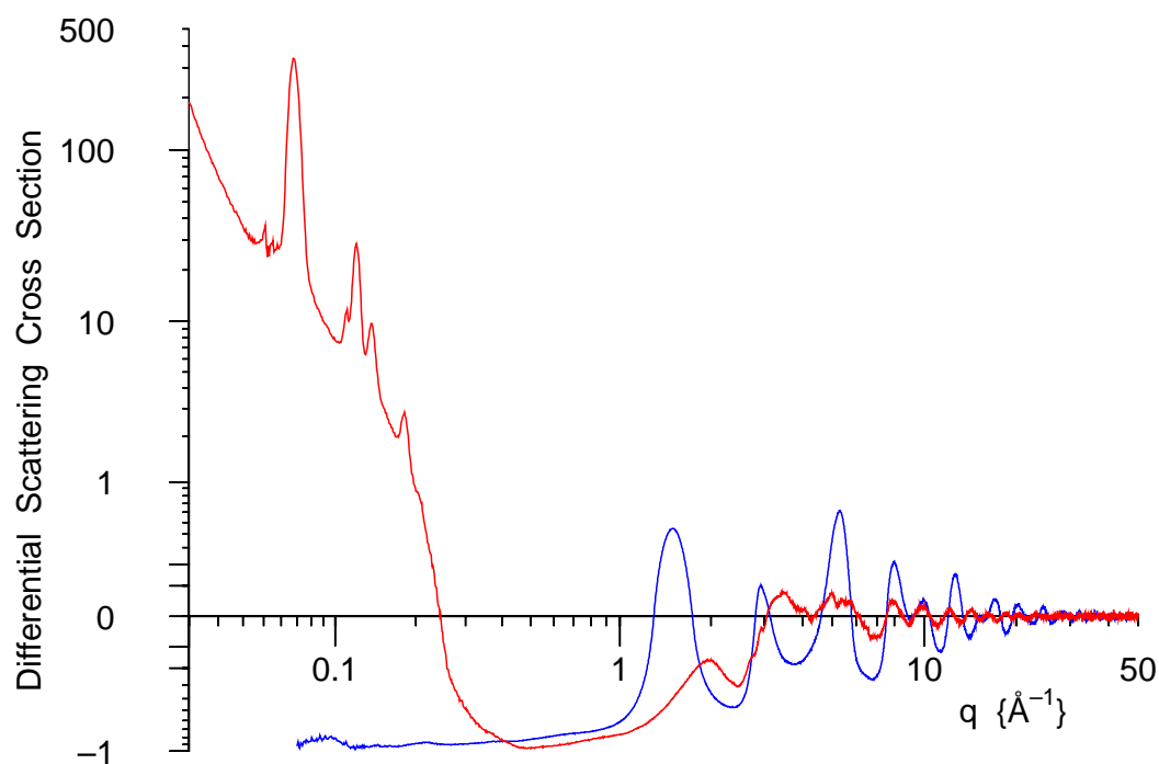
Figure 3. Differential Scattering Cross Section curves for a solid silica slab and a mesoporous SBA-15 silica.
