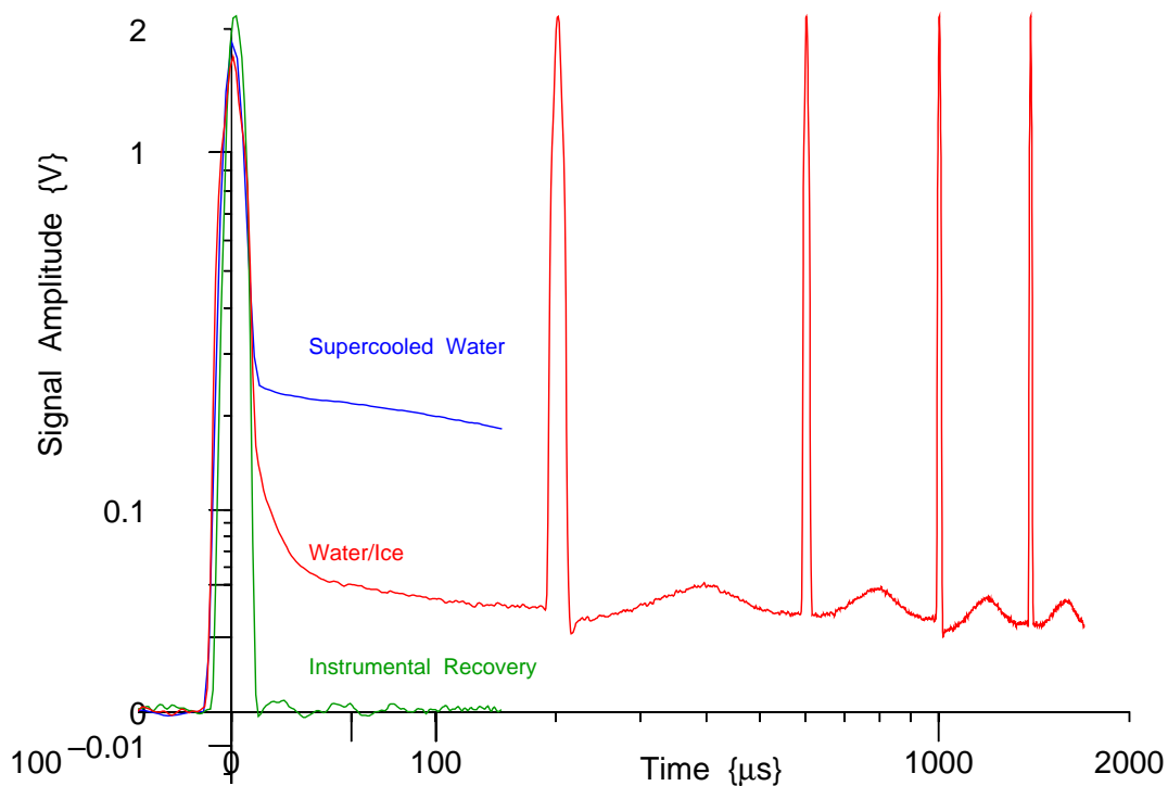
Figure 2. NMR cryoporometry signal traces for ice and water in mesoporous SBA-15 silica. Top curve: supercooled water at -5^\circ\text{C} . Lower curve: instrumental recovery - the signal from the NMR receiver, following the powerful 90^\circ NMR transmitter pulse, with no sample. Middle curve: signal from water/ice following freezing and re-warming to -5^\circ\text{C} : initial 10 \mu\text{s} T_2 free induction decay from bulk ice around silica grains, followed by a 4 ms T_2 decay defined by peaks of echoes, from the melted water in the pores.
