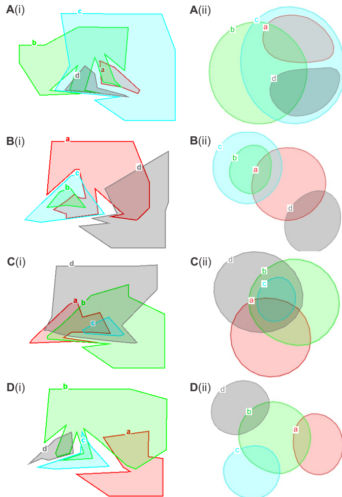
Fig. 3. Examples of (i) diagrams with four curves by Rodger et al.'s method [27] in our library and (ii) the correct layouts by eulerForce .
