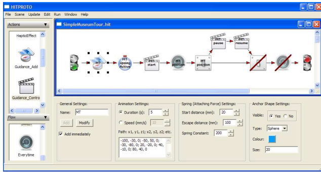
Figure 4: The museum tour interaction diagram: the user is led along a predefined path and at chosen points of interest, the tour is paused, to allow the user to explore the surroundings before resuming.
