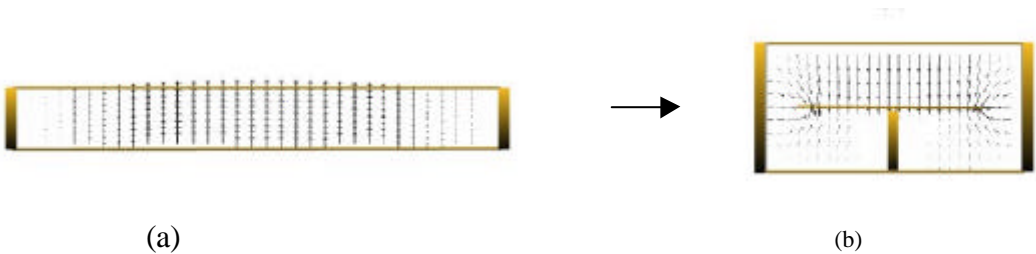
Fig. 1. Cross-sectional view of a standard waveguide (a) and folded waveguide (b)
