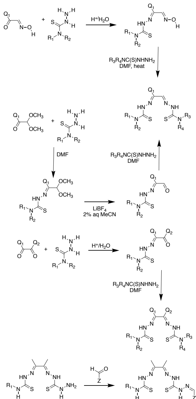
Fig. 2. Literature routes for synthesis of dissymmetric bis(thiosemicarbazone) pro-ligands using isonitronone or acetal protection and using unprotected diketones, and dissymmetric functionalisation via a thiocarbohydrazide side arm.
