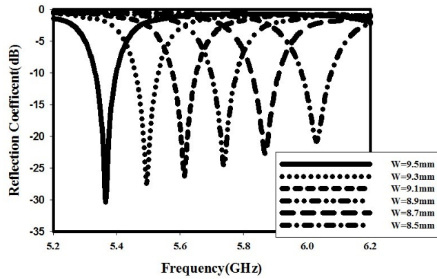
Figure 8. Reflection characteristics verses W ( L=40\text{mm} , a=16\text{mm} , H=0.254\text{mm} , W_s=1.2\text{mm} )
