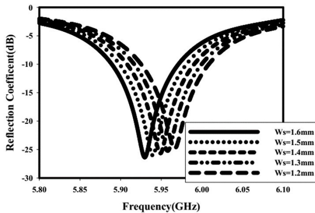
Figure 9. Reflection characteristics verses W_s ( L=40\text{mm} , a=16\text{mm} , W=8.613\text{mm} , H=0.254\text{mm} )
