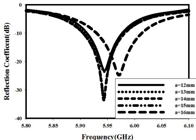
Figure 10. Reflection characteristics verses a ( L=40\text{mm} , H=0.254\text{mm} , W=8.613\text{mm} , W_s=1.2\text{mm} )
