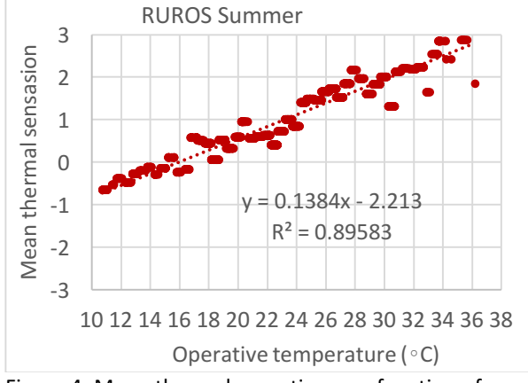
Figure 4: Mean thermal sensation as a function of operative temperature (°C) for the different studies
