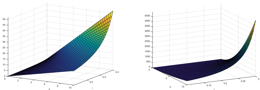
Figure 1: The left figure shows the limiting behaviour of the first moment when 0 < \theta < 10 and 0.1 < \gamma < 0.4 . The right figure shows the limiting behaviour of the first moment when 0 < \theta < 10 and 0.1 < \gamma < 0.3 .
