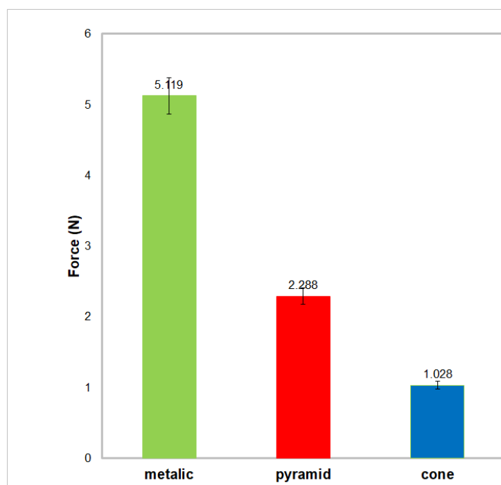
Fig. 6: Maximum forces for MN penetration in porcine skin.
