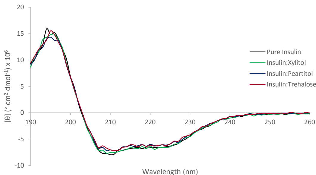
Fig. 3: CD of insulin and insulin formulations.
