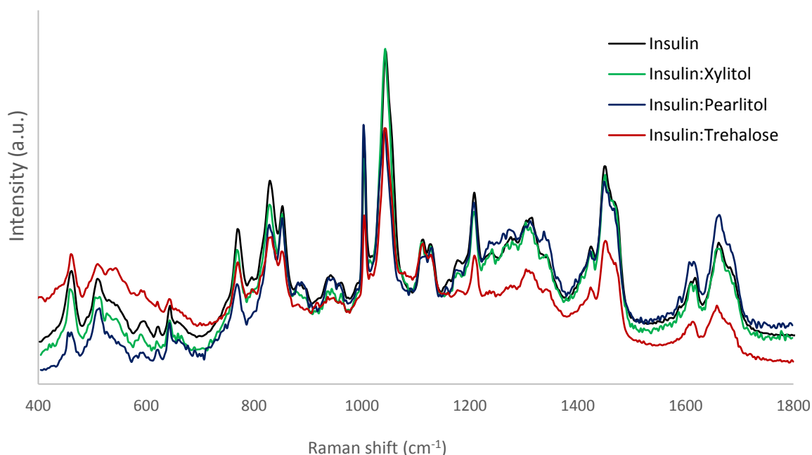
Fig.4: Raman spectra from 400 to 1800 cm -1 of pure insulin and insulin formulations.
