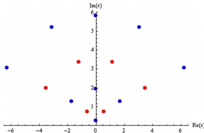
Figure 3. The 15 upper half plane zeros of F_5(x, 0) from the fifth-order rational solution. Poles of G_5/F_5 with residue +2i are marked with red dots, while those with residue -2i are marked with blue dots. This resembles a scaled version of figure 2 with an additional upper blue arc.
