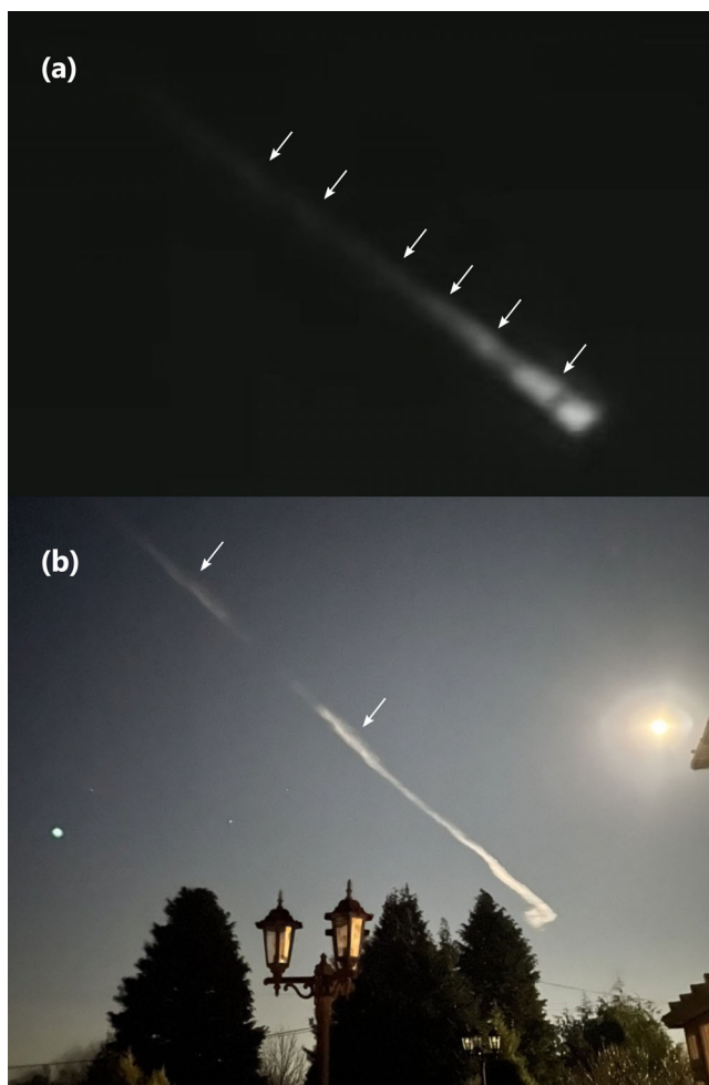
Fig. 12. Images of the Winchcombe fireball and trail. a) A frame from studio security camera footage over Midsomer Norton, UK of the Winchcombe fireball. Bright pulses of plasma within the trail are labeled by arrows. b) A photograph of the persistent trail illuminated by the full moon, as seen from Ruardean Hill, Gloucestershire. © Daniel M. ( imo.net ).
