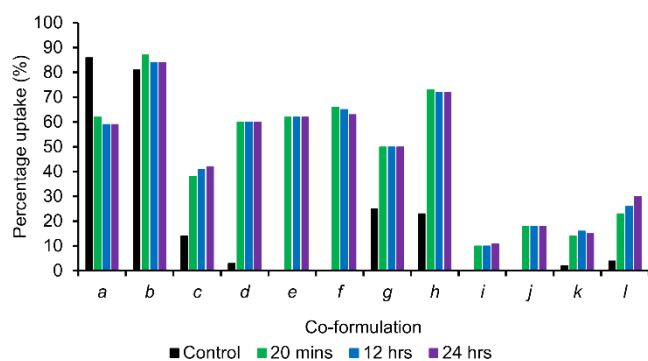
Figure 3 Graph comparing the percentage uptake of co-formulant into preformed SSA self-associated structures of 1-3 and 5 over a 24-hour period at 298 K and a concentration of 5.56 mM. Here the control data set represents the percentage of co-formulant incorporated into SSA self-associated structures as they were formed. Experiments involving co-formulations a-h were undertaken in a \text{D}_2\text{O}/\text{EtOH} 19:1 solutions, whereas
