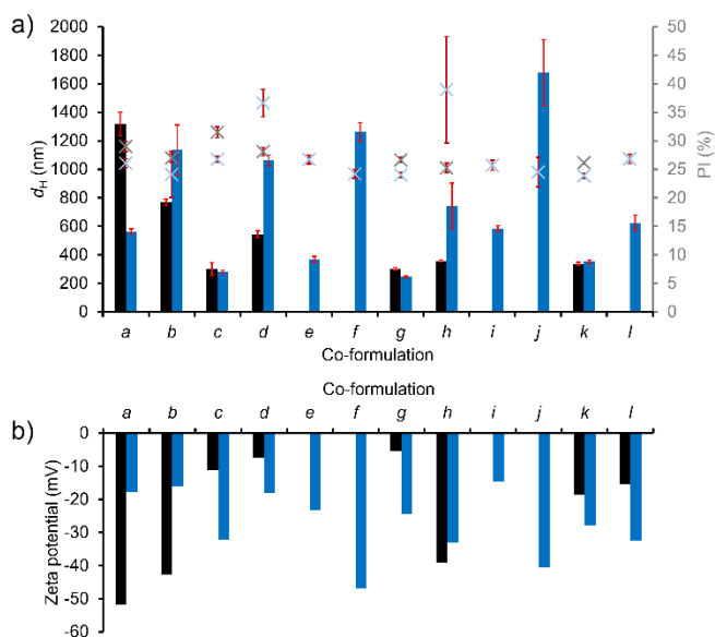
Figure 4 Summary of a) DLS (bars) and associated polydispersity index values (crosses) and b) Zeta potential measurements for co-formulations a-l conducted produced through institute formation (Black/grey) or after 20 minutes post addition to pre-formed SSA aggregated species (Blue) at a concentration of 5.56 mM in a H 2 O/EtOH 19:1 solution at 298 K.
