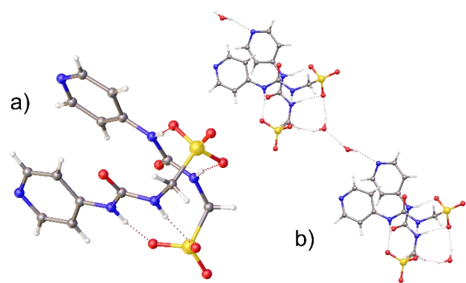
Figure 2 Single crystal X-ray structure obtained for SSA 3 showing: a) an anionic SSA dimer, stabilised through the formation of four intermolecular hydrogen bonds; and b) the extended hydrogen bonded network where the SSA anion dimers are connected through the presence of intermolecular hydrogen bonded water molecules. Where appropriate the H 2 O and TBA counter-cations have been omitted for clarity. Grey = carbon, blue = nitrogen, red = oxygen, yellow = sulfur, white = hydrogen, red dashed lines = hydrogen bonds. † The presence of the urea-sulfonate hydrogen bonded dimer is promoted by the presence of the weakly coordinating, comparatively hydrophobic TBA counter-cation. 20
