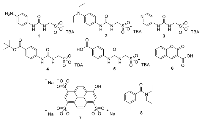
Figure 1 Chemical structures of SSAs 1–5 and co-formulants 6–8.
