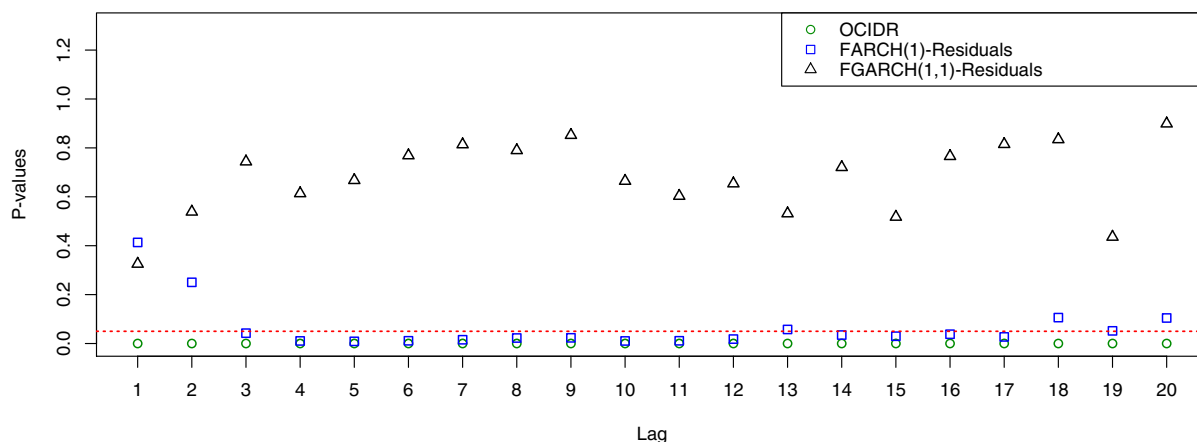
Figure 4. P -values of white noise and goodness of fit tests for the FARCH(1) and FGARCH(1,1) models applied to the OCIDR curves derived from the S&P 500 index based on M_{N,K,\epsilon} as a function of K , K = 1, \dots, 20 . The horizontal red line is at the level of 5%. The plot generally suggests the adequacy of the FGARCH(1,1) model [Color figure can be viewed at wileyonlinelibrary.com]
