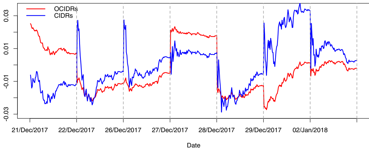
Figure 3. Plots of de-volatized S&P 500 intra-day return curves based on an FGARCH(1,1) Model from 21 December 2017 to 2 January 2018 [Color figure can be viewed at wileyonlinelibrary.com ]
