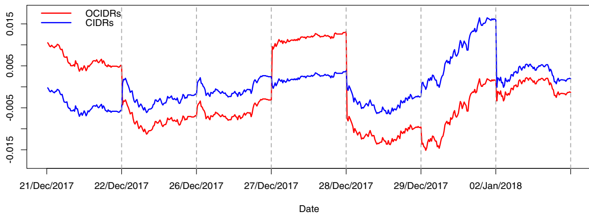
Figure 1. Plots of cumulative and overnight cumulative intra-day log return curves of S&P 500 from 21 December 2017 to 2 January 2018 [Color figure can be viewed at wileyonlinelibrary.com ]
