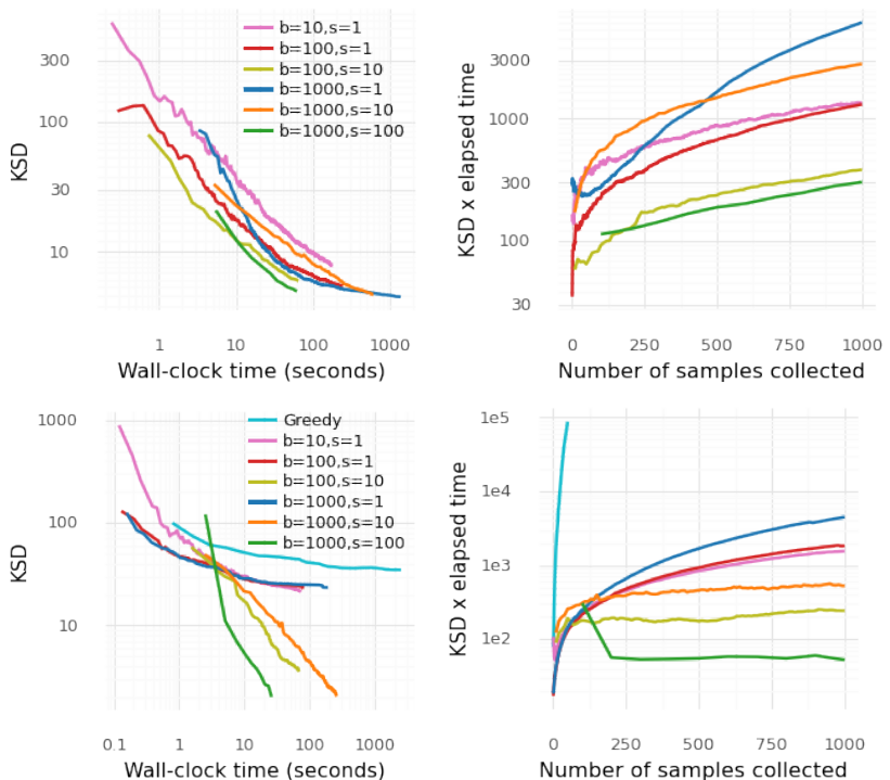
Figure 3: KSD vs. wall-clock time, and KSD \times time vs. number of selected samples, shown for the 38-dim calcium signalling model (top two panes) and 4-dim Lotka–Volterra model (bottom two panes). The kernel length-scale in each case was set using the median heuristic (Garreau et al., 2017), and estimated in practice using a uniform subsample of 1000 points for each model. The myopic algorithm of Riabiz et al. (2020) is included in the Lotka–Volterra plots—see main text for details.
