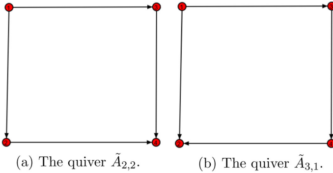
Fig. 5 Two orientations of the A_3^{(1)} Dynkin diagram
