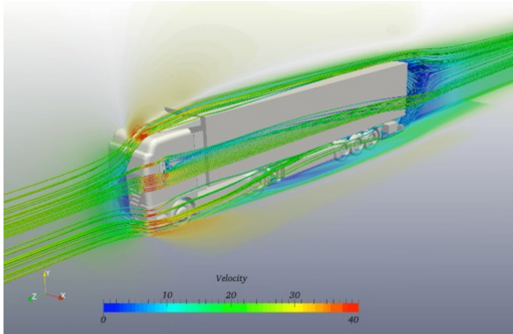
Figure 3.1.1 CFD simulation of a HGV and trailer travelling at 28m/s
