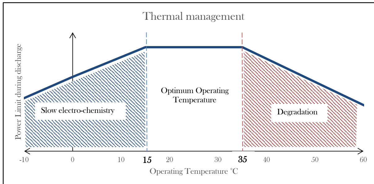
Figure 5.3.4 Thermal Management for Lithium-Ion Batteries in an EV. (This graph was created based on data found here: http://www.nrel.gov/docs/fy13osti/58145.pdf )
