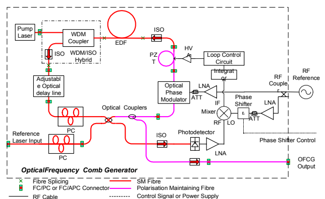
Figure 1. Dual coupler configuration OFCG with a fiber stretcher to stabilize the comb.
