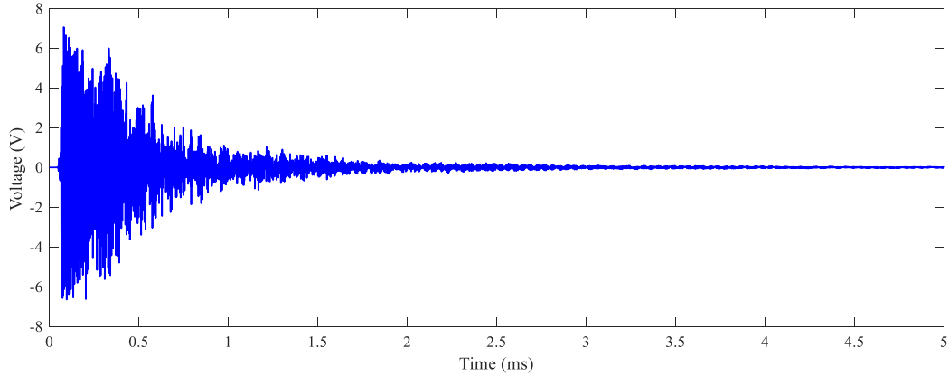
Fig. 8. Typical AE signal from an individual collision (particle diameter 0.8 mm and impact velocity 32 m/s).
