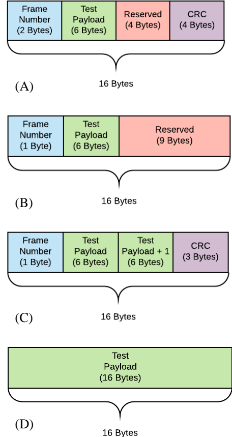
Fig. 4. System Frame Types
