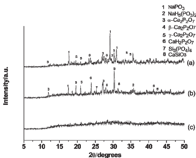
Fig. 11 (a) P45Ca20Na20Si15, (b) P45Ca30Na10Si15, (c) P45Ca40Si15 at 600 °C.
