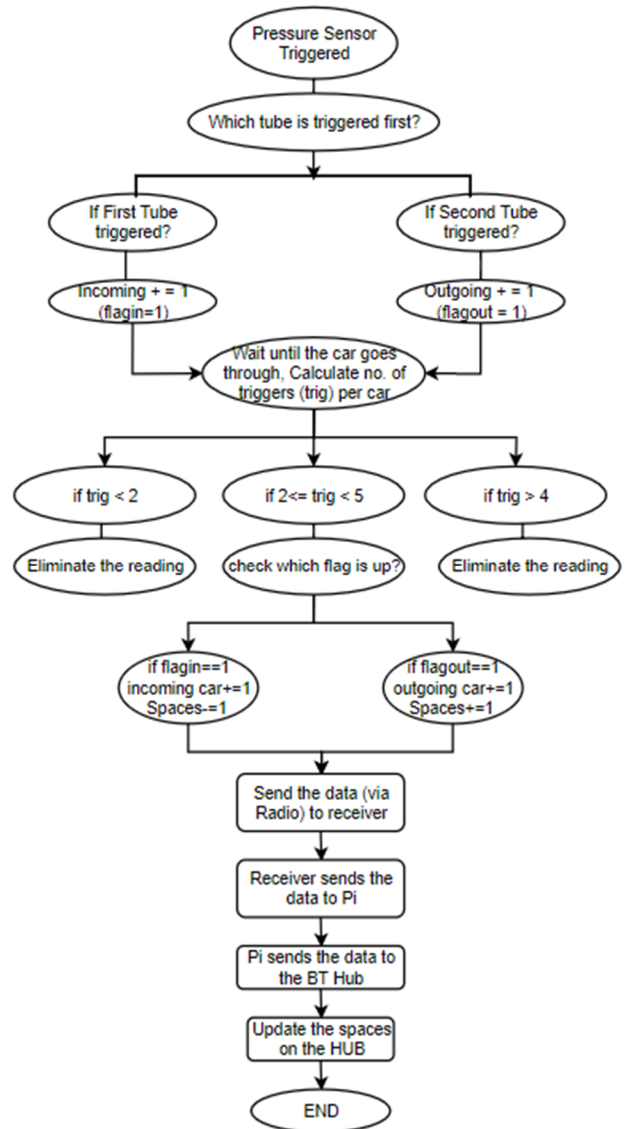
Figure 7 Algorithm Design
