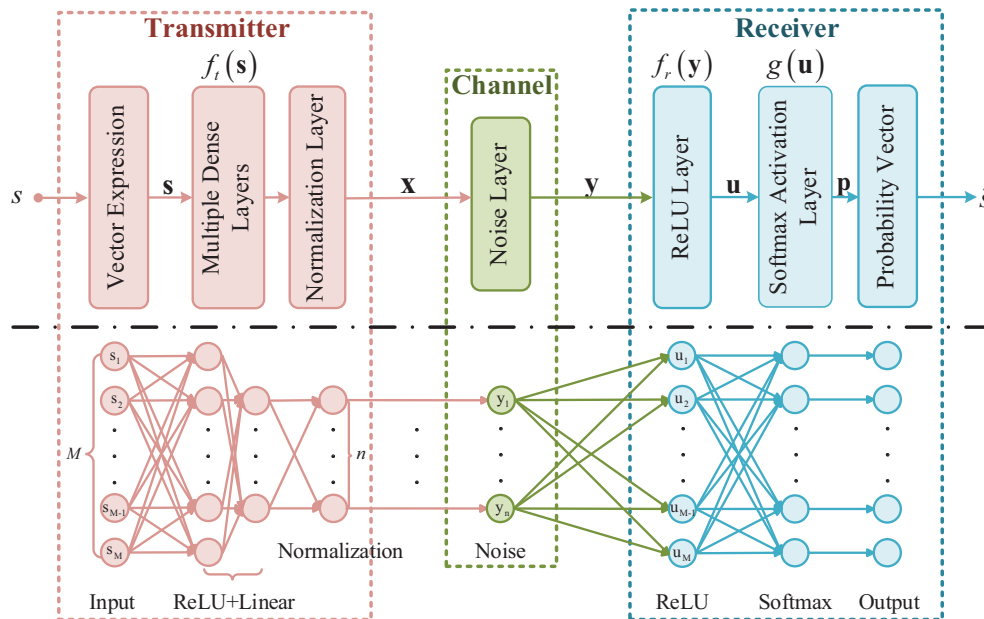
Fig. 1. A DL-based communication system represented as an autoencoder with its NN structure [19].
