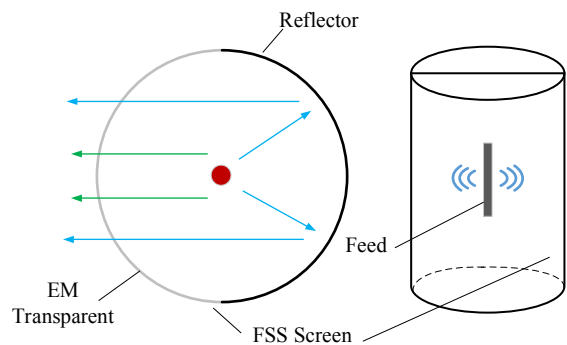
Figure. 1. The operation principle of the AFSS antenna.
