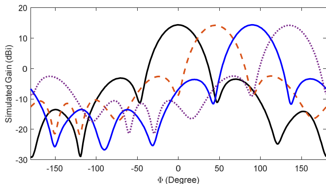
Figure 6. Simulated beam-switching radiation patterns of the high-gain AFSS antenna at 3.5GHz.
