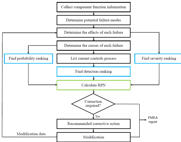
Fig 2– FMEA process.
