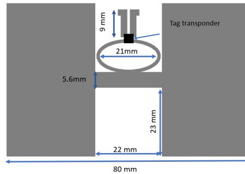
Fig. 1. Vapor Sensing Tag Design
