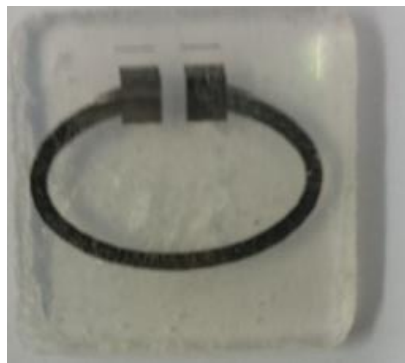
Fig. 2. Inkjet Printed Conductive Loop on PDMS Block
