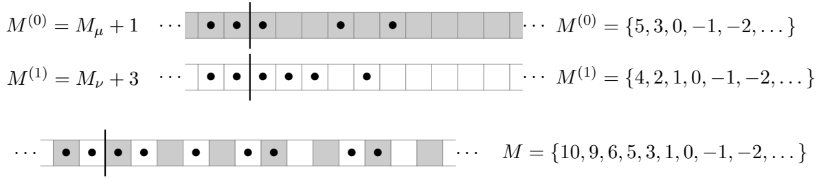
Figure 4: The Maya diagrams corresponding to Example 1.
