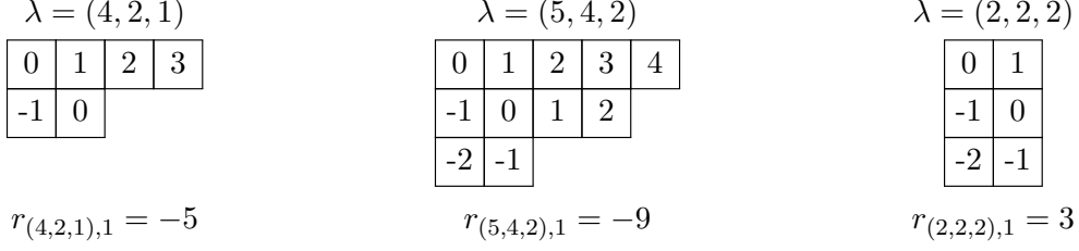
Figure 7: Examples of the values r_{\lambda,1} where the boxes of the Young diagrams contain the respective contents.
