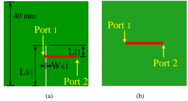
Fig. 4. (a) Configuration of the proposed half-power phase shifter. Detailed parameters: L_{s1}=19 mm, W_{s1}=0.5 mm, L_{f1}=5.9 mm. (b) The traditional microstrip phase delay line.
