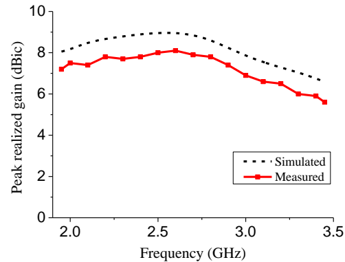
Fig. 17. Measured and simulated peak realized gain of the proposed differentially fed CP antenna.
