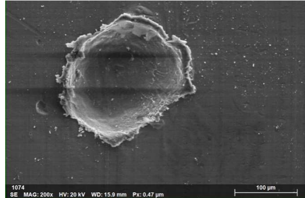
Figure 1: Example SEM secondary electron image of a crater formed following the impact of an ice particle at 1.5 \text{kms}^{-1} .
