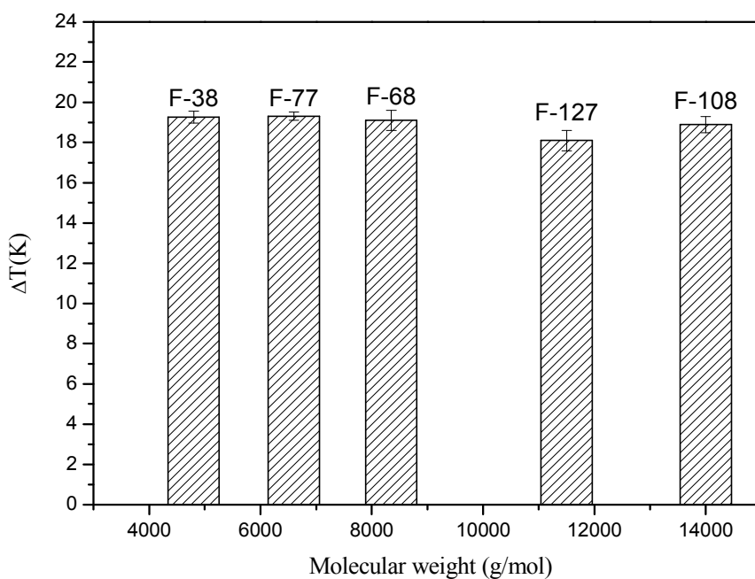
Figure 5: Comparison of melting point depression of Pluronic® with molecular weight where, ( \Delta T = T_m measured by DSC – T_m at 30 MPa).
