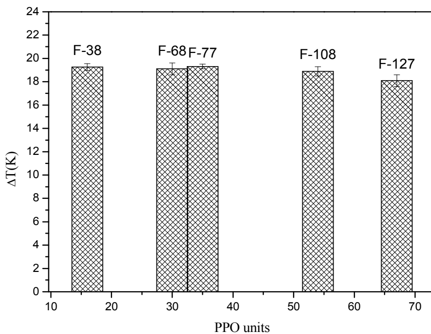
Figure 6: Comparison of melting point depression of Pluronic® with PPO units where, ( \Delta T = T_m measured by DSC – T_m at 30 MPa).
