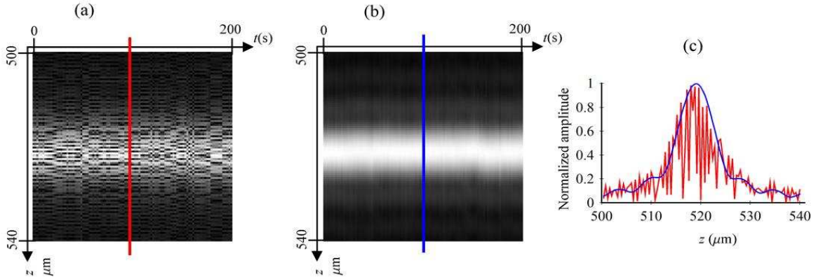
Fig. 2. (a) A-scans (vertical axis) for a mirror as object, represented in time (horizontal axis) calculated with MSI and 100 CS_{\text{exp}} utilized as masks. (b) A-scans (vertical axis) for a mirror as object represented in time (horizontal axis) calculated with CMSI using 100 inferred masks obtained from 2 CS_{\text{exp}} . (c) Reflectance profiles calculated by MSI (red) and CMSI (blue) in a time t = 100 seconds.
