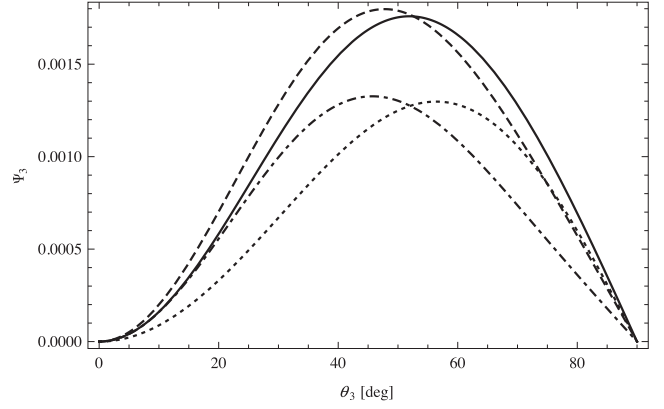
Figure 5. \Psi_3(\theta_3) for a spheroid with h = ca = 0.9 . Solid line: present solution, dashed: volume-scaled Efroimsky & Lazarian (2000), dotted: Molina et al. (2003); dot-dashed: re-derived Sharma et al. (2005) for the equivalent Q definition.
